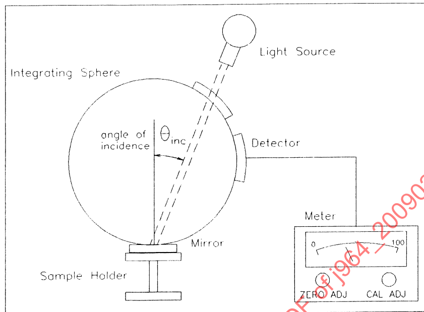
FIGURE 1—SCHEMATIC OF REFLECTOMETER WITH A FIXED RECEIVER AND A SAMPLE HOLDER WHICH LOCATES THE SAMPLE DIRECTLY ADJACENT TO THE SPHERE. THIS UNIT CAN BE USED TO MEASURE TOTAL REFLECTANCE OF FLAT AND NON-FLAT MIRRORS.
