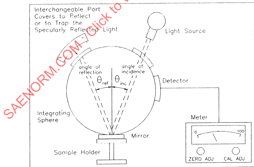
FIGURE 2—SCHEMATIC OF A REFLECTOMETER WITH THE MEANS FOR EXCLUDING THE SPECULARLY REFLECTED BEAM. THIS UNIT COULD BE USED FOR MEASURING TOTAL REFLECTANCE OF FLAT AND NON-FLAT MIRRORS, AND DIFFUSE REFLECTANCE OF FLAT MIRRORS.
