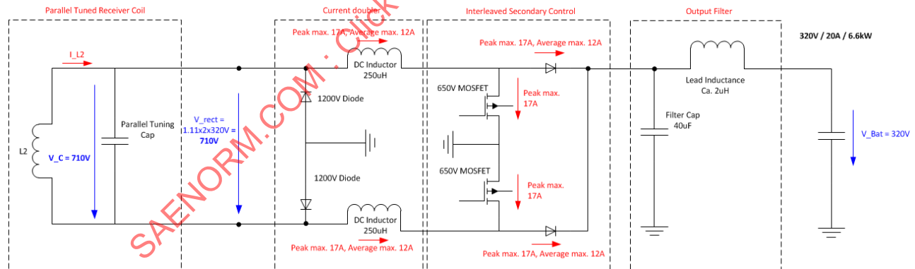
Figure G3 - Electrical specification of the Product VA WPT2/Z1
