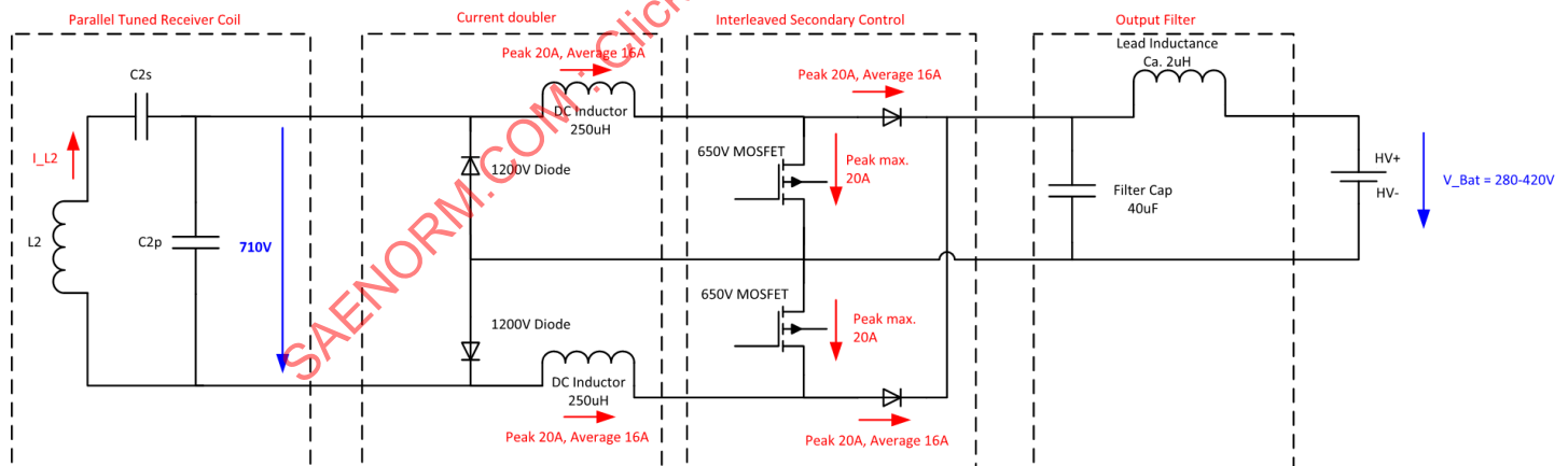
Figure G15 - Electrical specification of the Product VA WPT3/Z2.
