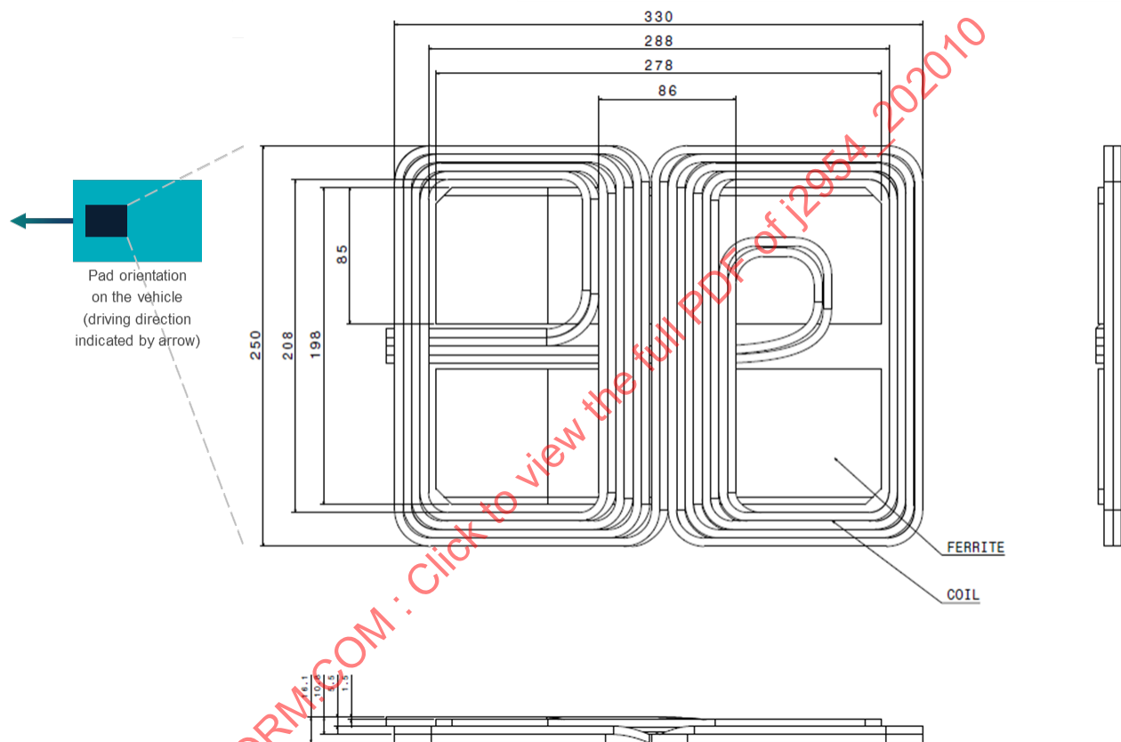
Figure G4 - Mechanical dimensions of the Product VA WPT2/Z2
