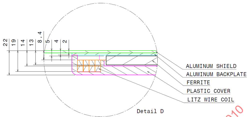
Figure G5 - Detailed cross-section view of the Product VA WPT2/Z2
