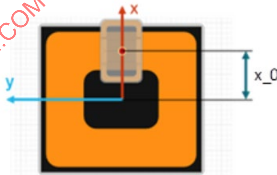
Figure 22 - Example for the “natural offset” definition x_0 for a DD-topology VA over a circular-topology GA
