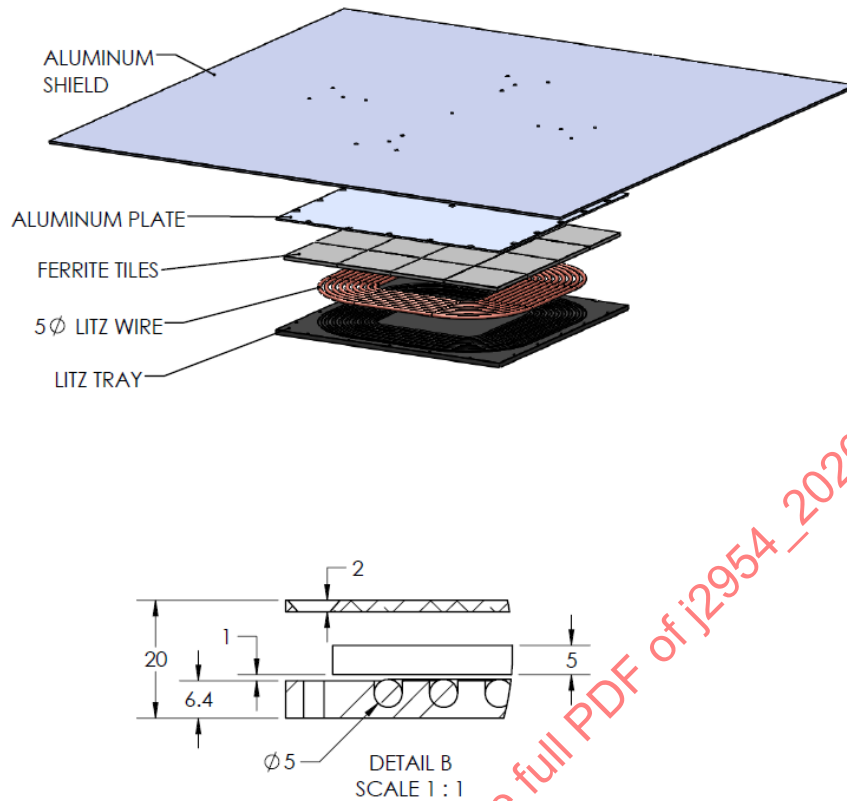
Figure A20 - Exploded view of the Test Station VA WPT2/Z2
