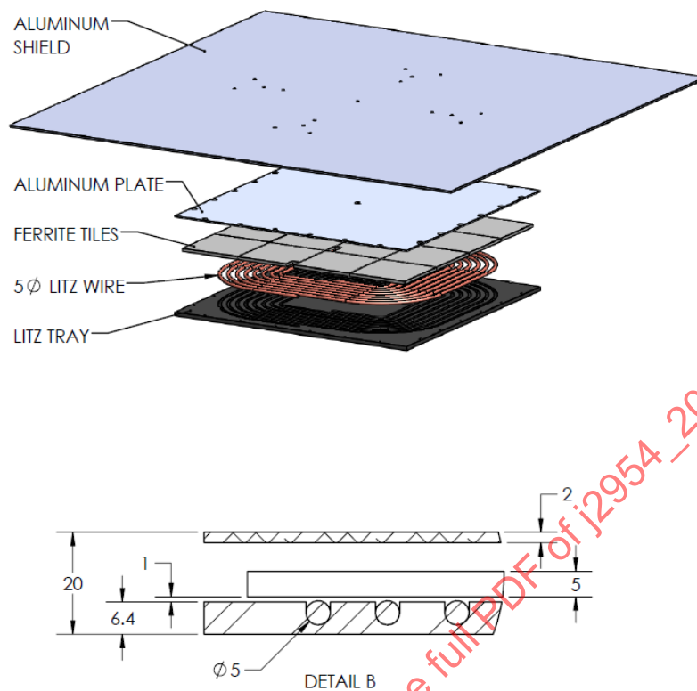
Figure A23 - Exploded view of the Test Station VA WPT2/Z3
