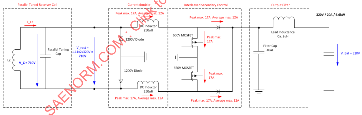
Figure G9 - Electrical specification of the Product VA WPT2/Z3
