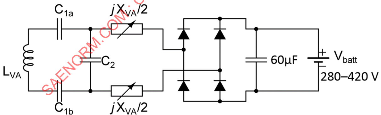
Figure A21 - Electrical specification of the Test Station VA WPT2/Z2.
