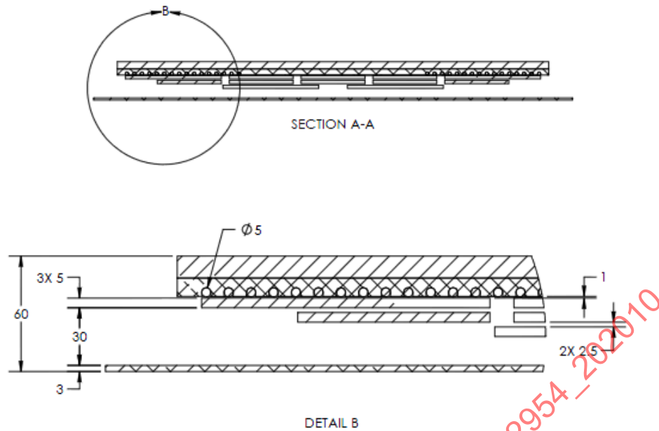
Figure B2 - Detailed cross section view of the Test Station Universal GA
