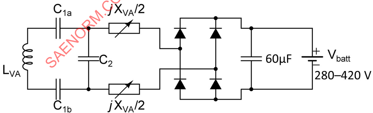
Figure A18 - Electrical specification of the Test Station VA WPT2/Z1
