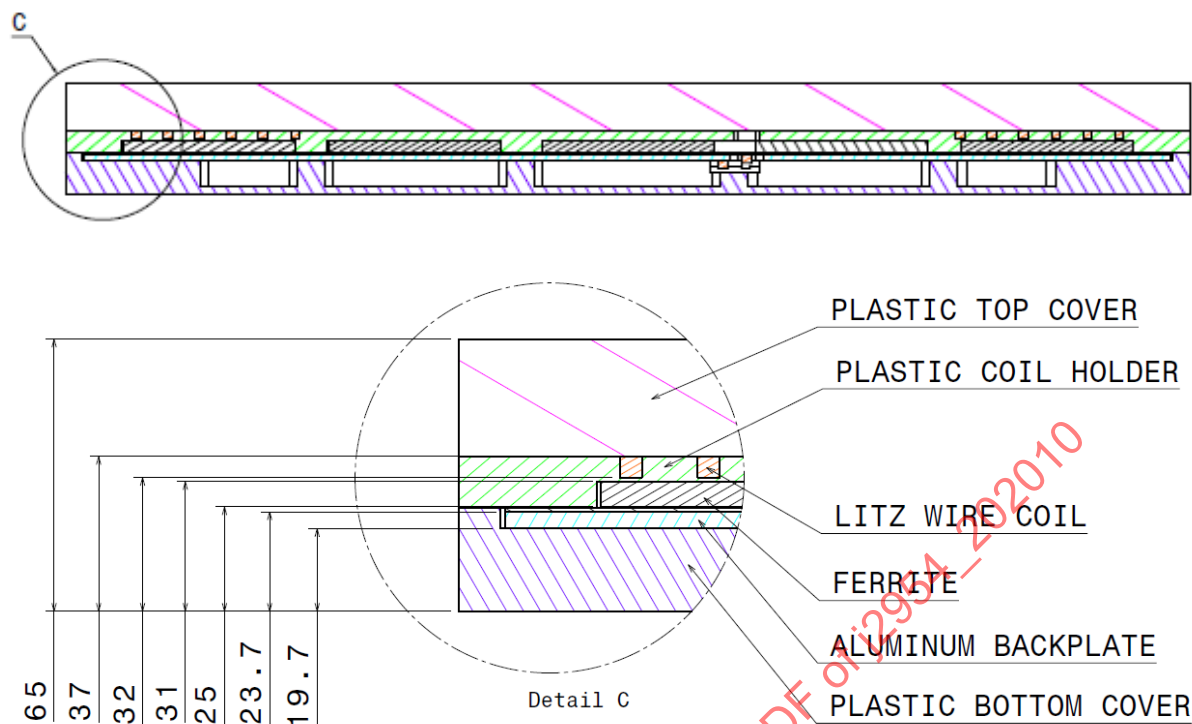
Figure H2 - Detailed cross-section view of the Product GA WPT2
