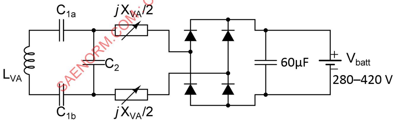
Figure A24 - Electrical specification of the Test Station VA WPT2/Z3
