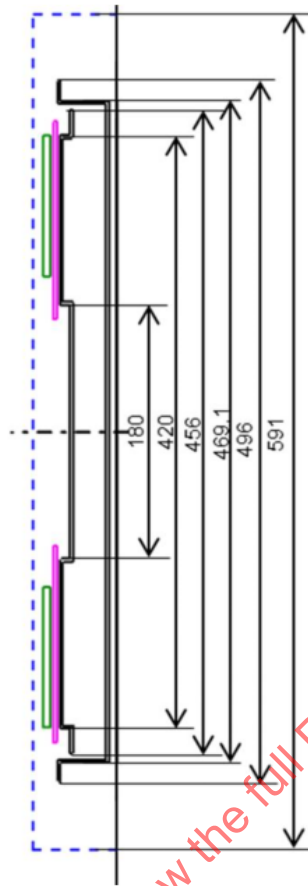
Figure F2 - Mechanical dimensions of the GA WPT1
