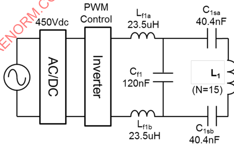
Figure F6 - Electrical specification of the GA WPT1
