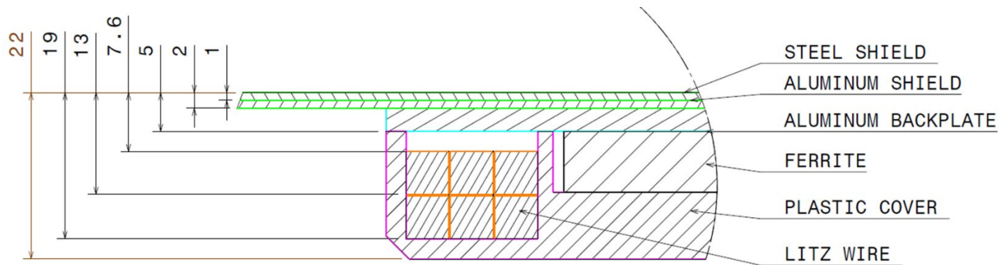
Figure G17 - Detailed cross-section view of the Product VA WPT3/Z3
