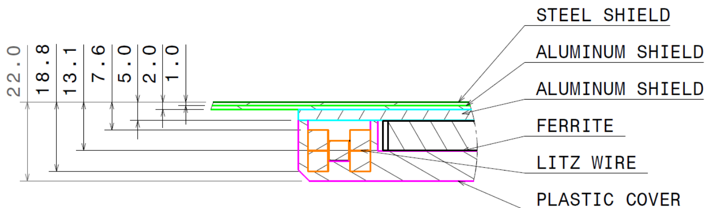
Figure G11 - Detailed cross-section view of the Product VA WPT3/Z1
