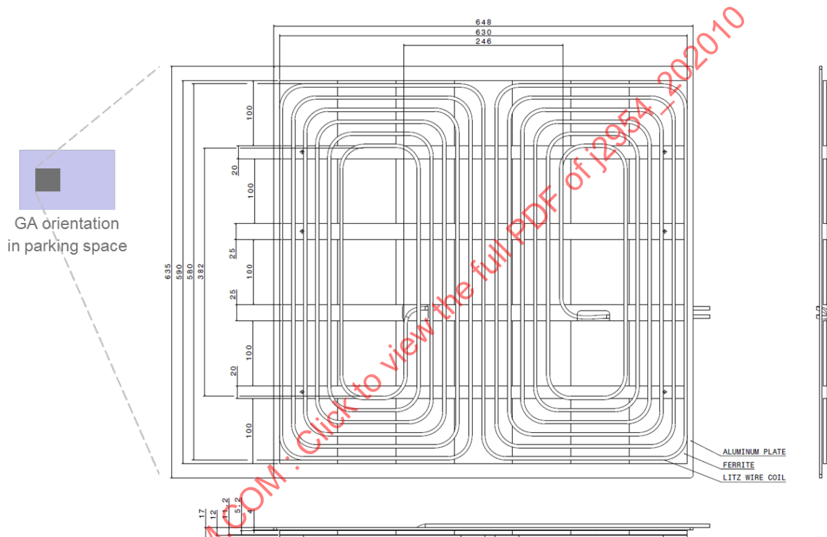
Figure H1 - Mechanical dimensions of the Product GA WPT2
