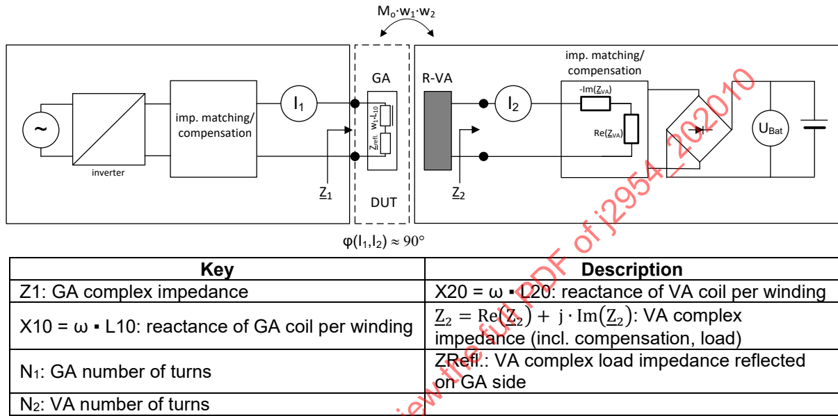
Figure J2 - Schematic to explain impedance
