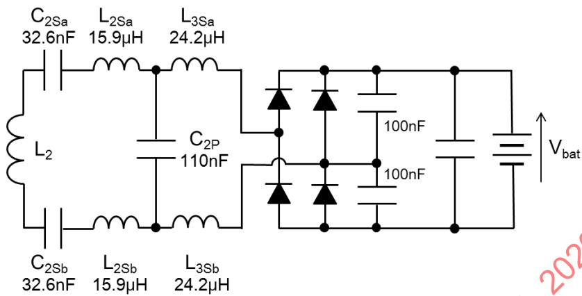
Figure A5 - Electrical specification of the Test Station VA-WPT1/Z1
