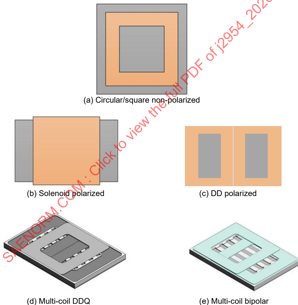
Figure I1 - Common assembly topologies
