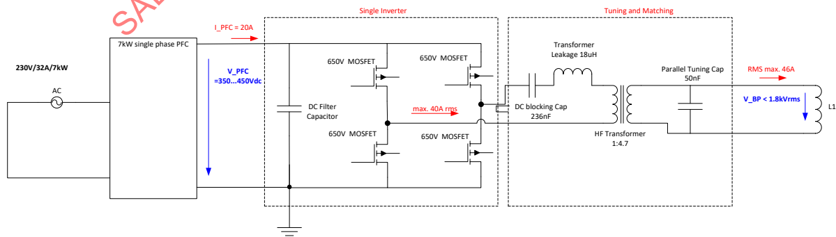
Figure H3 - Electrical specification of the Product GA WPT2
