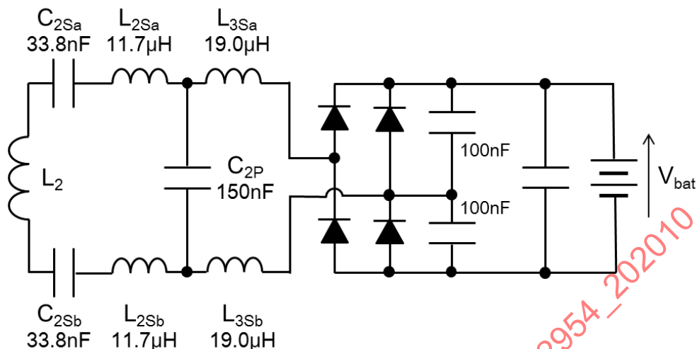
Figure A15 - Electrical specification of the Test Station VA-WPT1/Z3
