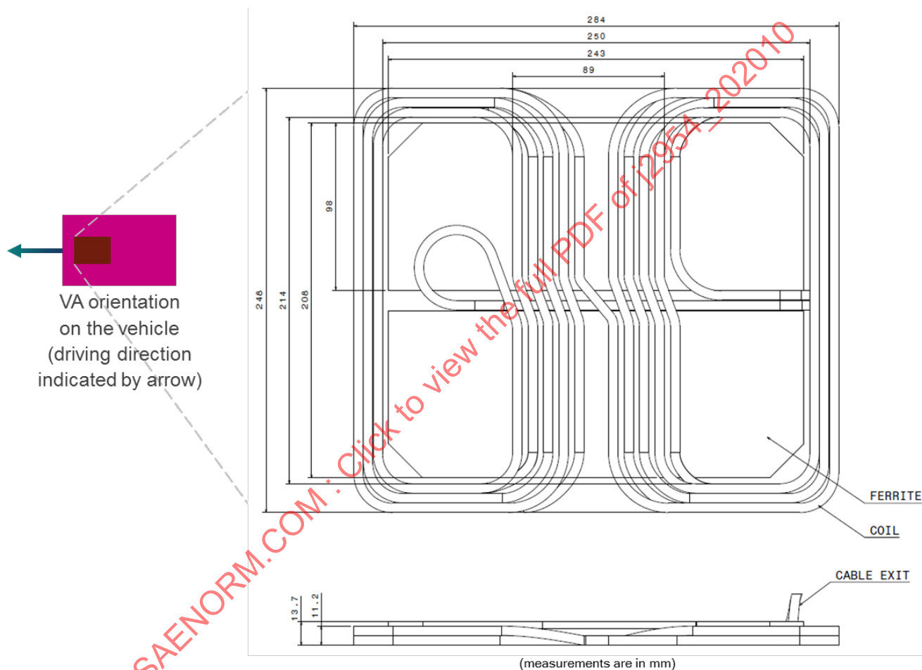
Figure G10 - Mechanical dimensions of the Product VA WPT3/Z1
