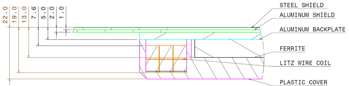
Figure G14 - Detailed cross-section view of the Product VA WPT3/Z2
