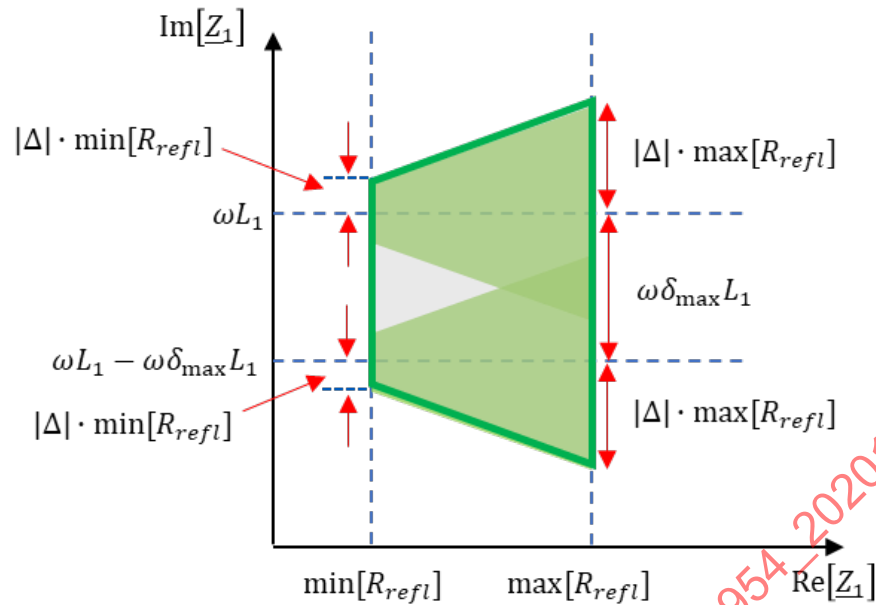
Figure J4 - Impedance space at the GA coil (example)
