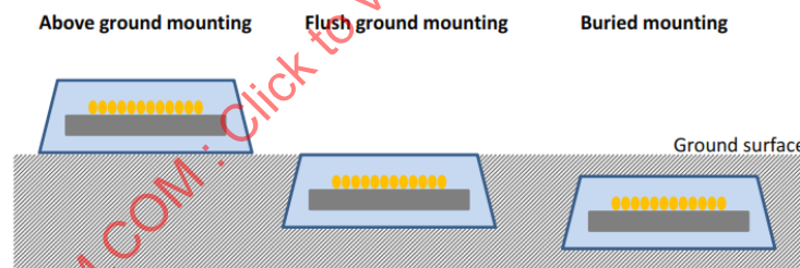
Figure 3 - GA mounting schemes
