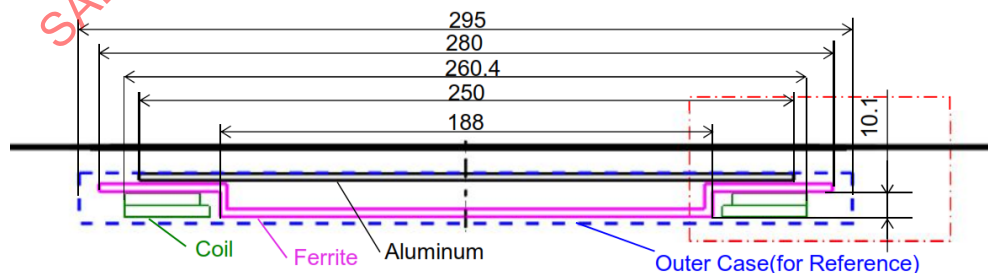
Figure A2 - Mechanical dimensions of the Test Station VA WPT1/Z1
