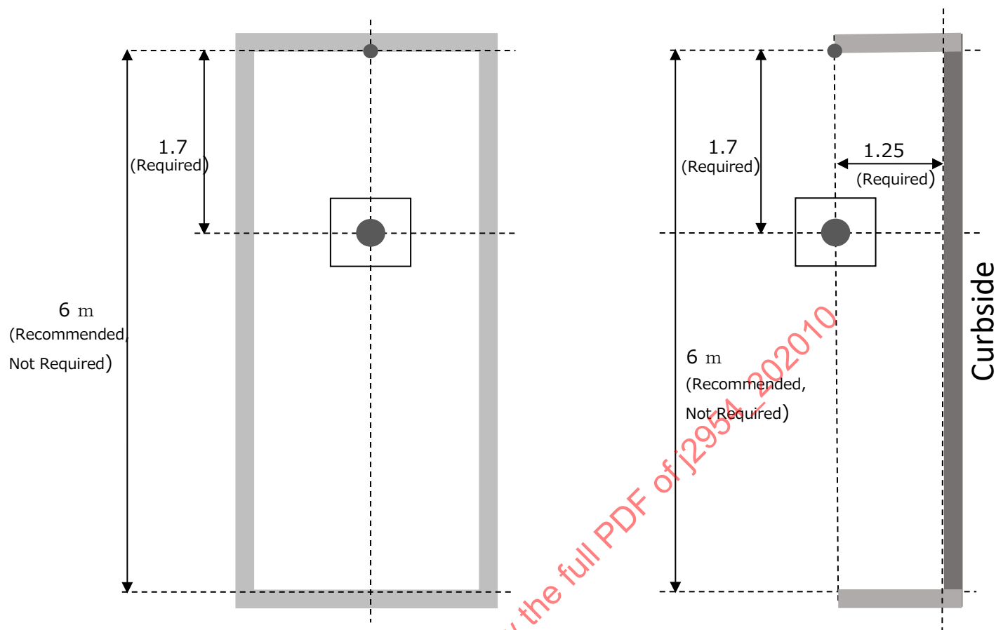
Figure 24 - SAE J2954 GA geometric center location diagram
