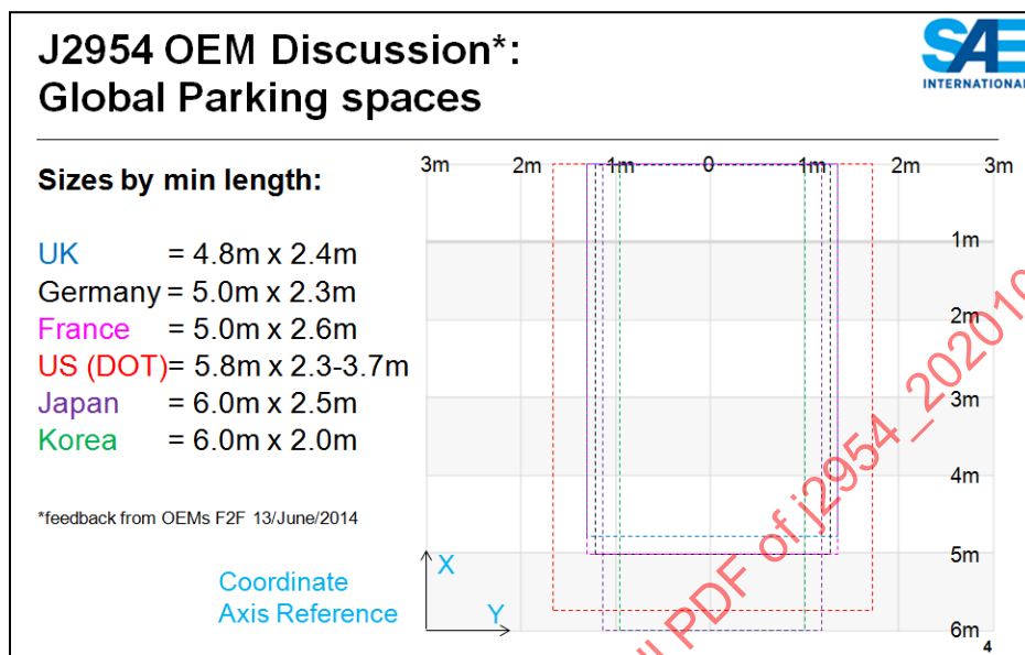
Figure D1 - SAE J2954 OEM survey for GA location in parking space
