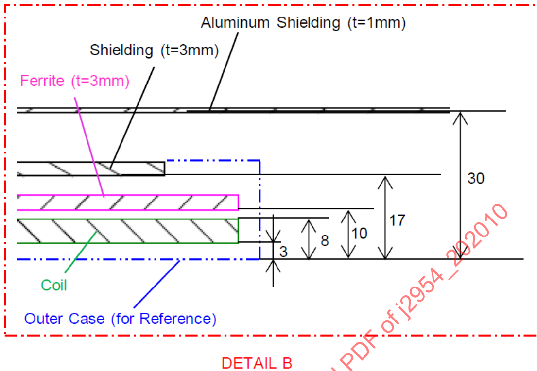
Figure A13 - Detailed cross section view
