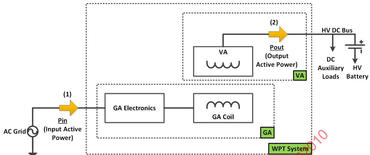
Figure 28 - Block diagram of a WPT system (including VA and GA) illustrating the efficiency points (1) and (2)
