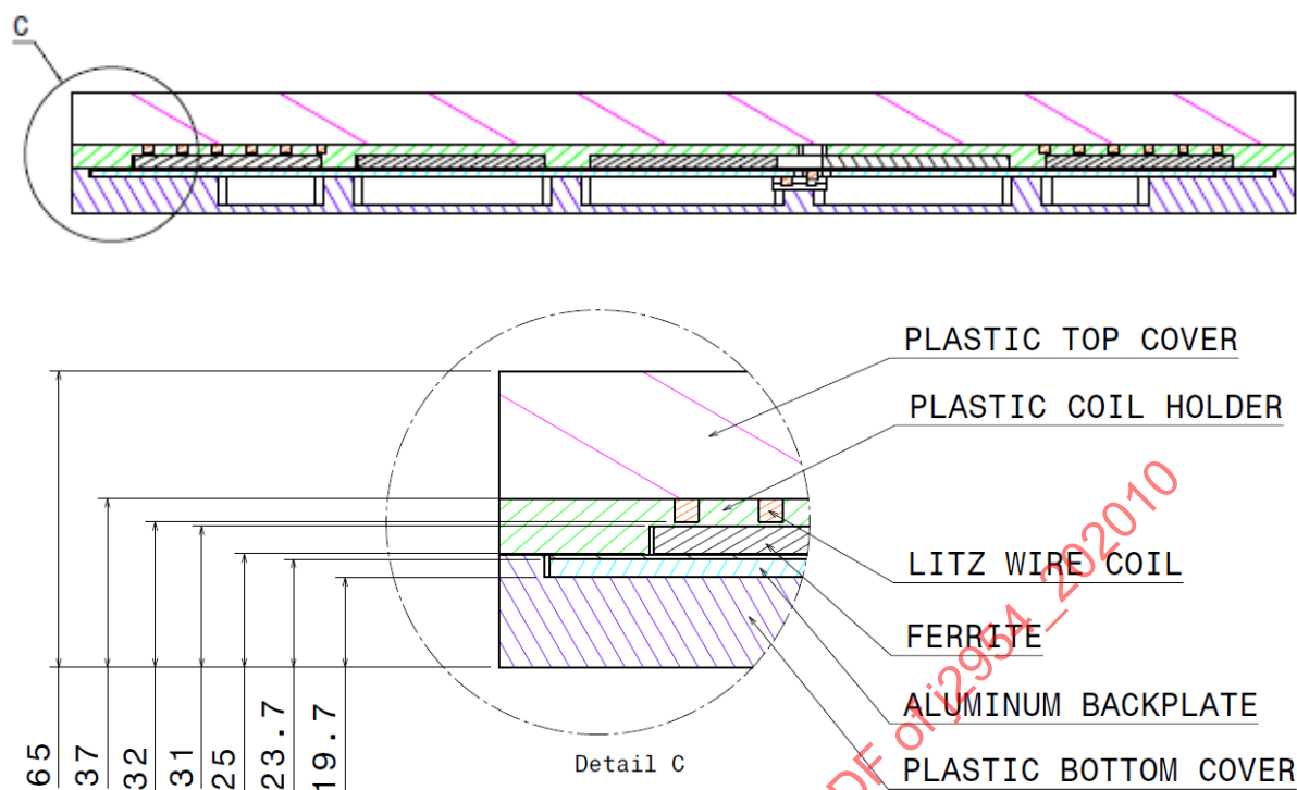
Figure H5 - Detailed cross-section view of the Product GA WPT3
