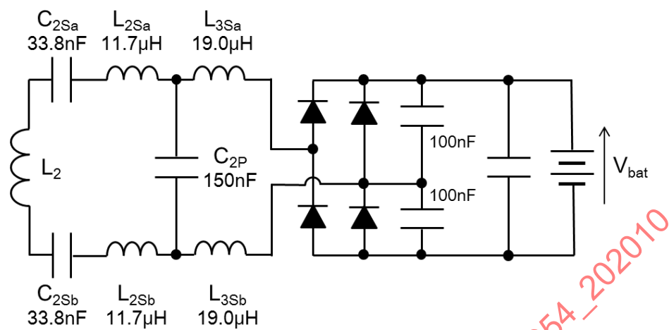
Figure A10 - Electrical specification of the Test Station VA-WPT1/Z2
