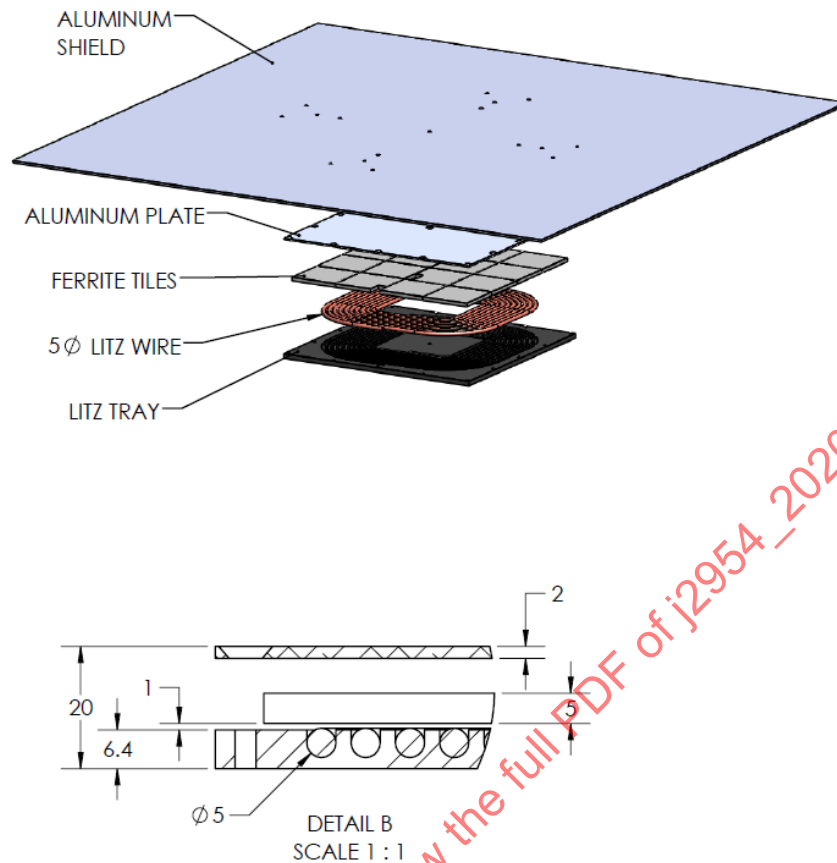
Figure A17 - Exploded view of the Test Station VA WPT2/Z1
