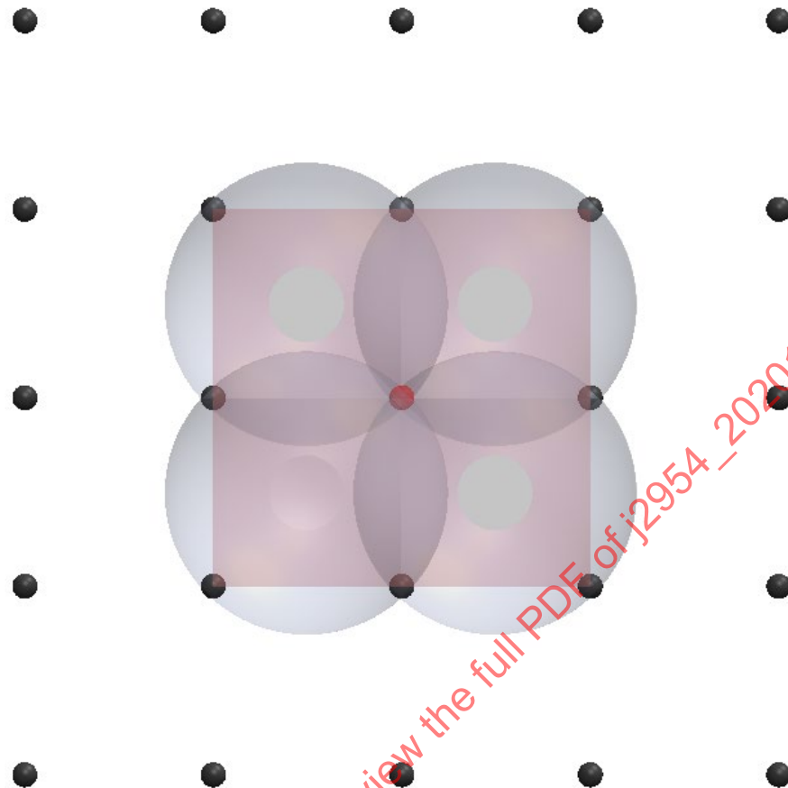
Figure 18 - Locations for standard field probe averages around peak - 2 x 2 grid separated equidistantly by 7.5 cm center-to-center
