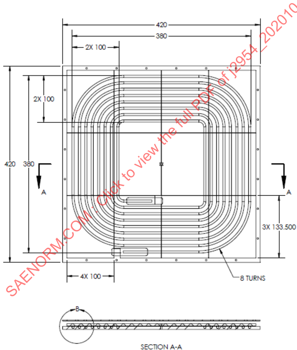
Figure A31 - Mechanical dimensions of the Test Station VA WPT3/Z3
