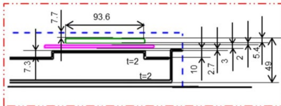
Figure F4 - Detailed cross-section view
