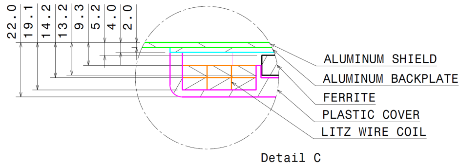
Figure G8 - Detailed cross-section view of the Product VA WPT2/Z3
