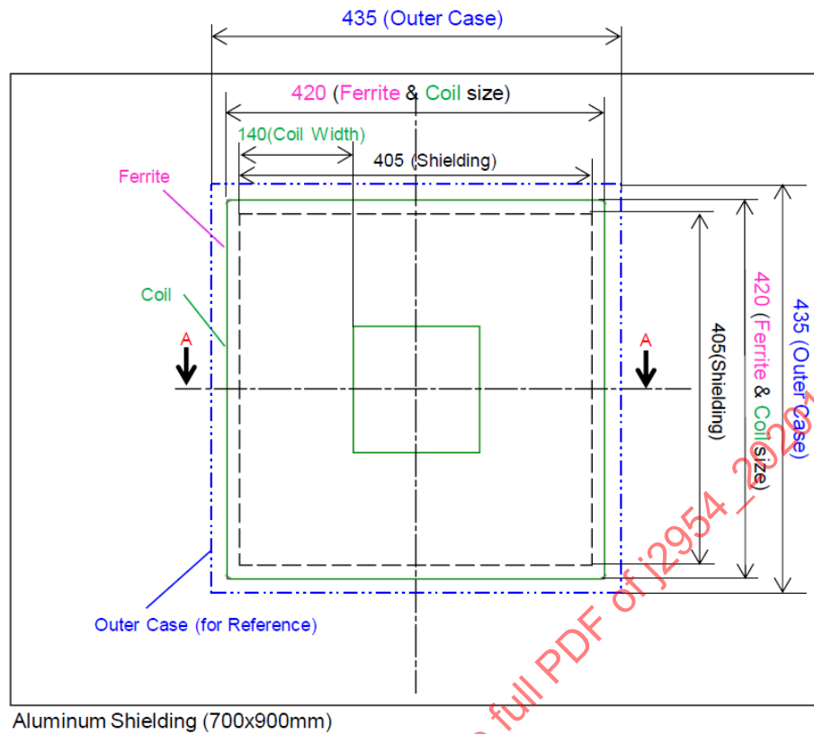
Figure A11 - Mechanical dimensions of the Test Station VA WPT1/Z3
