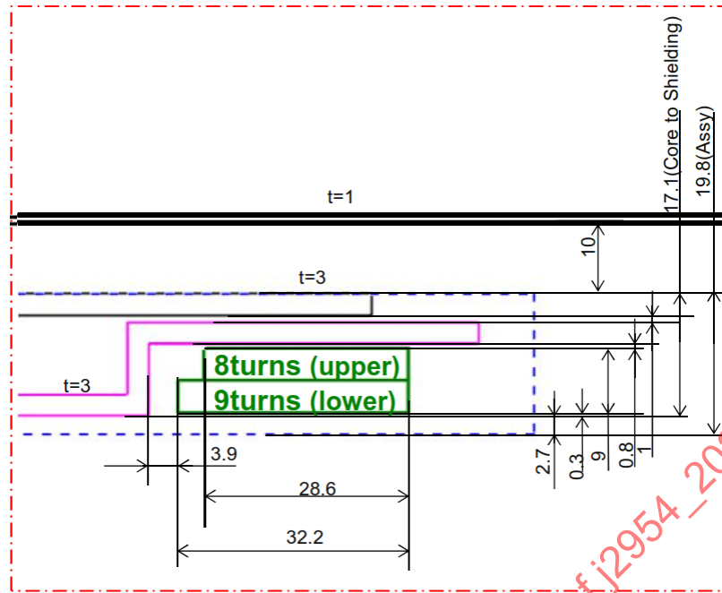
Figure A3 - Detailed cross section view
