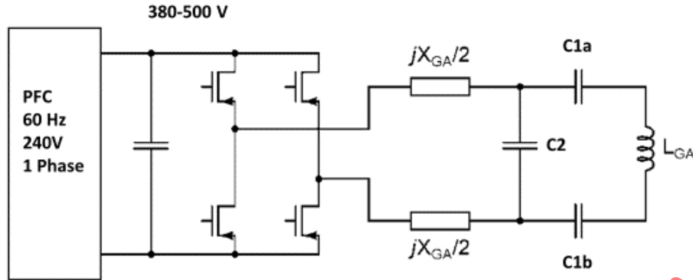
Figure B4 - Electrical schematic of the Test Station Universal GA
