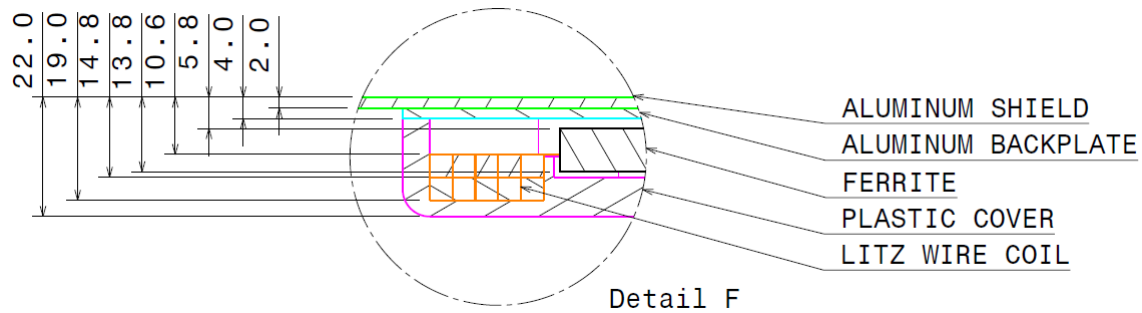
Figure G2 - Detailed cross-section view of the Product VA WPT2/Z1
