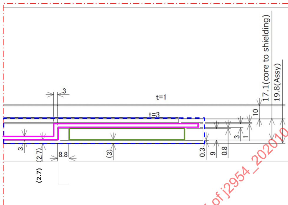
Figure A8 - Detailed cross section view
