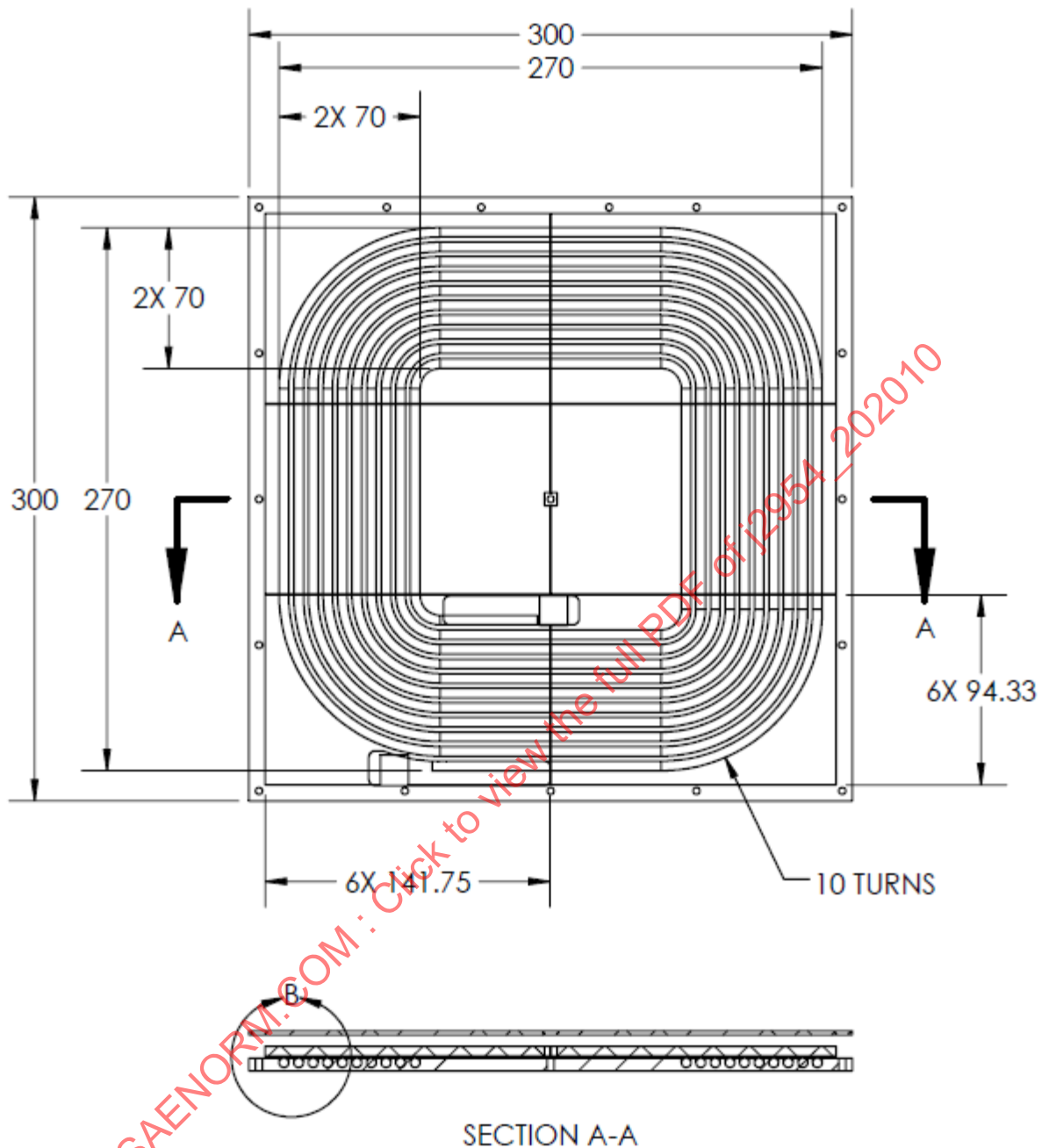
Figure A25 - Mechanical dimensions of the Test Station VA WPT3/Z1
