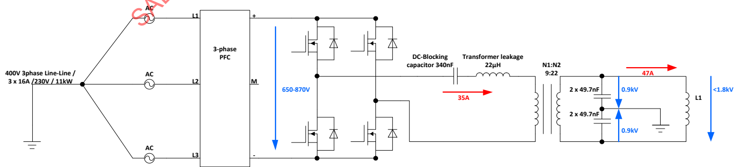
Figure H6 - Electrical specification of the Product GA WPT3
