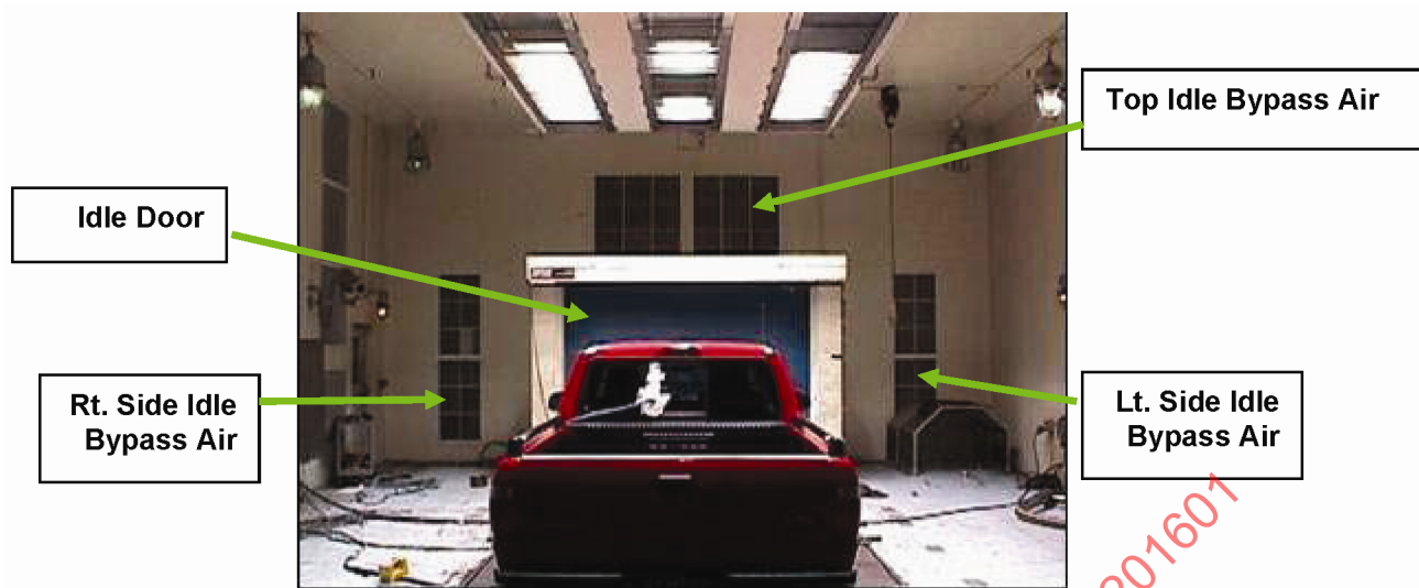
Figure 11 - Vehicle in wind tunnel showing bypass air configuration
