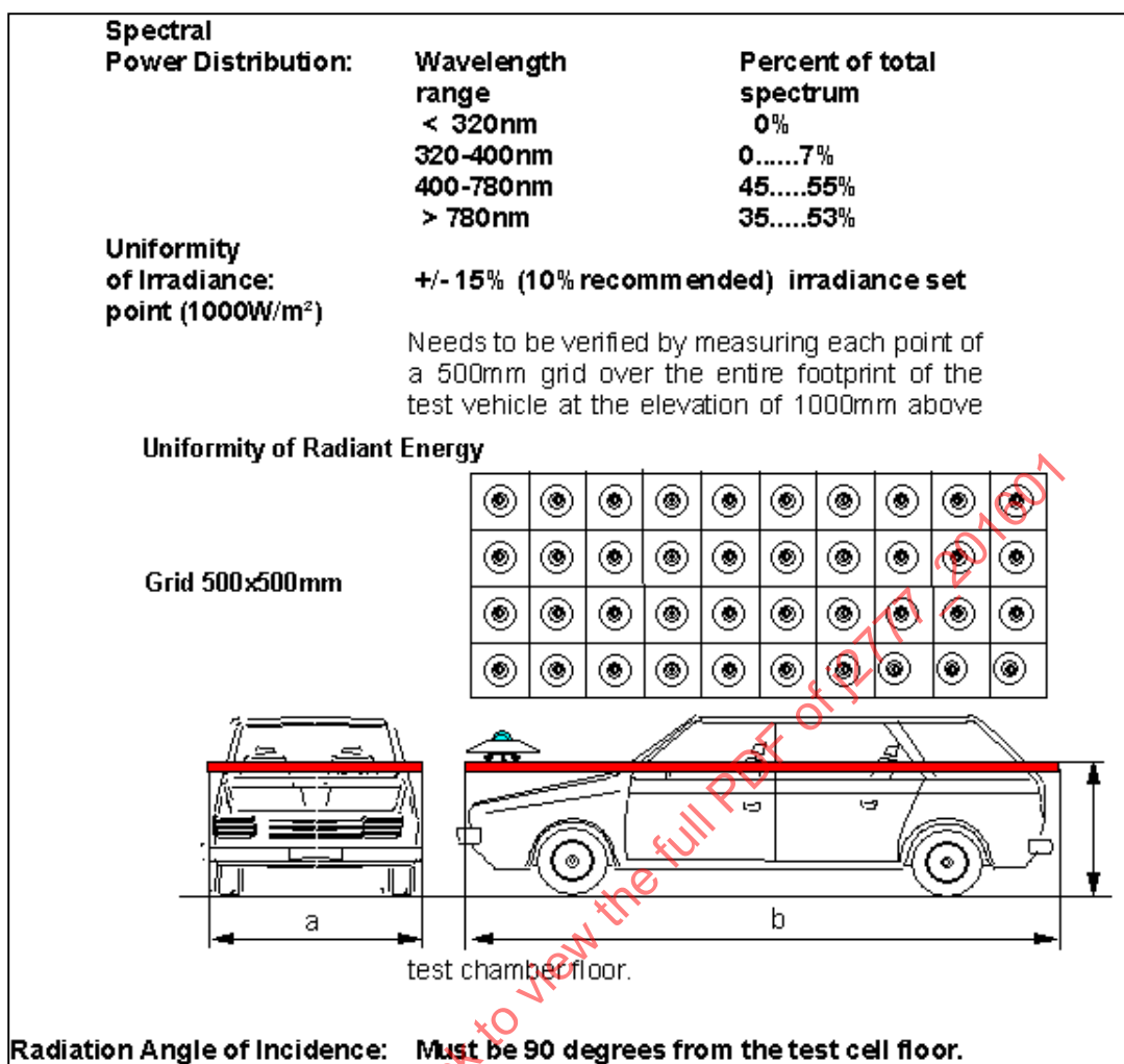
Figure 7 - Recommended solar simulation distribution
