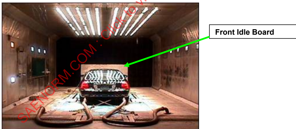
Figure 12 - Vehicle in wind tunnel with air bypass air using idle board
