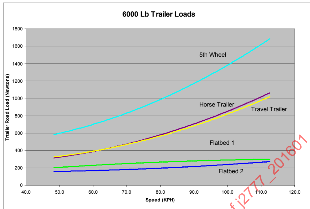
Figure 3 - Variability in trailer road load forces with the same trailer weight
