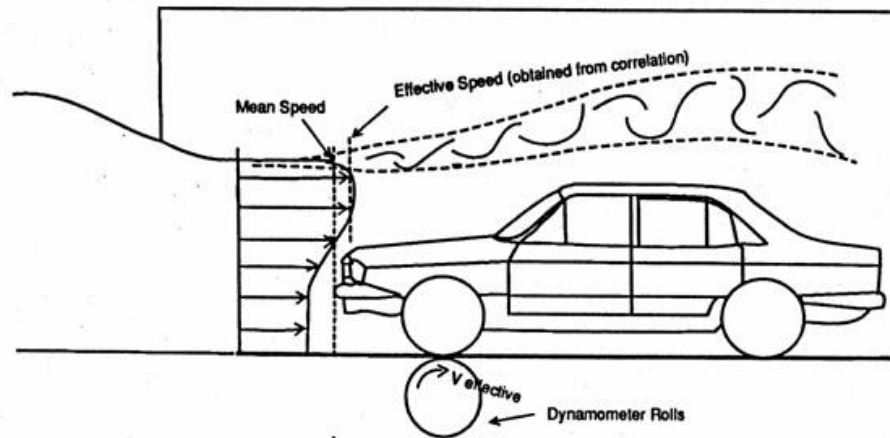
Figure 5 - Wind tunnel velocity profile
