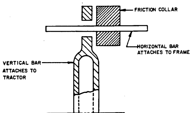
FIG. 13—TYPICAL METHOD OF MEASURING DEFLECTION
