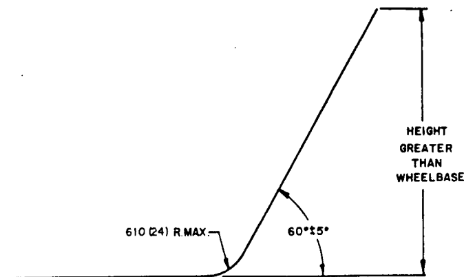
FIG. 14—TYPICAL REAR OVERTURN BANK
