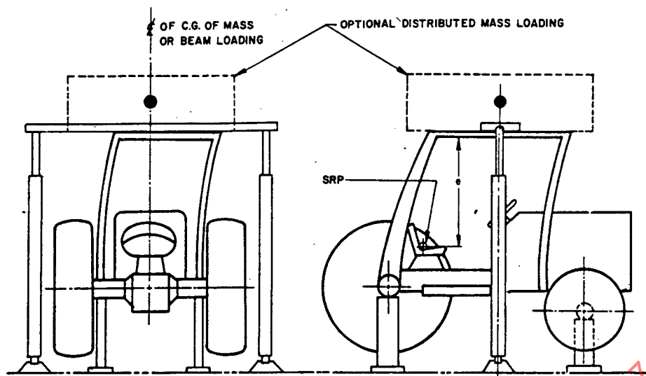
FIG. 7—TYPICAL METHOD OF LOAD APPLICATION FOR CRUSH TEST
