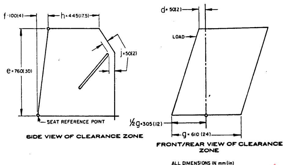
FIG. 12—PICTORIAL REPRESENTATION OF CLEARANCE ZONE
