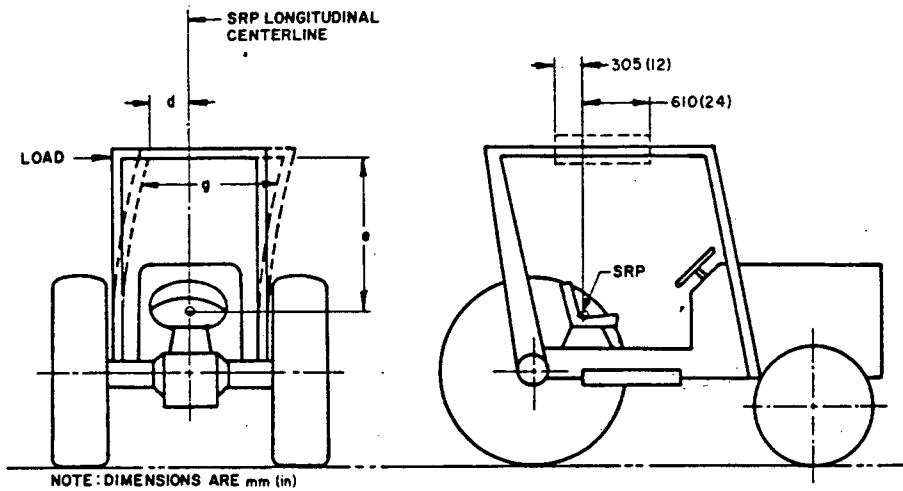
FIG. 6—TYPICAL SIDE LOAD APPLICATION
