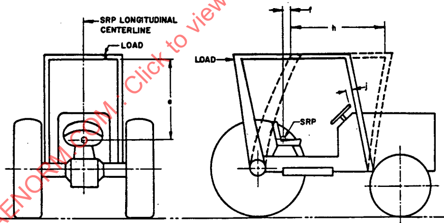
FIG. 5—TYPICAL REAR LOAD APPLICATION
