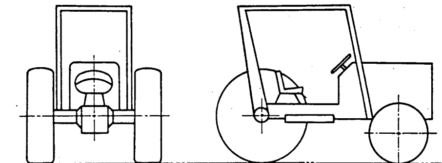
FIG. 2—TRACTOR WITH TYPICAL 4-POST ROPS
