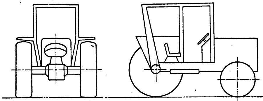
FIG. 3—TRACTOR WITH TYPICAL PROTECTIVE ENCLOSURE
