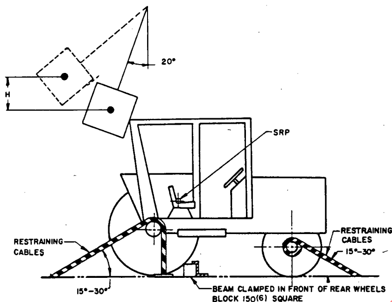
FIG. 10—TYPICAL REAR IMPACT APPLICATION
