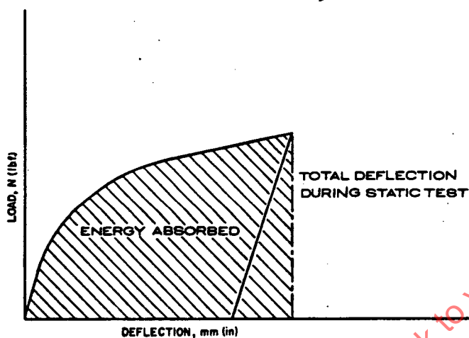
FIG. 8—FORCE DEFLECTION (F-D) CURVE
