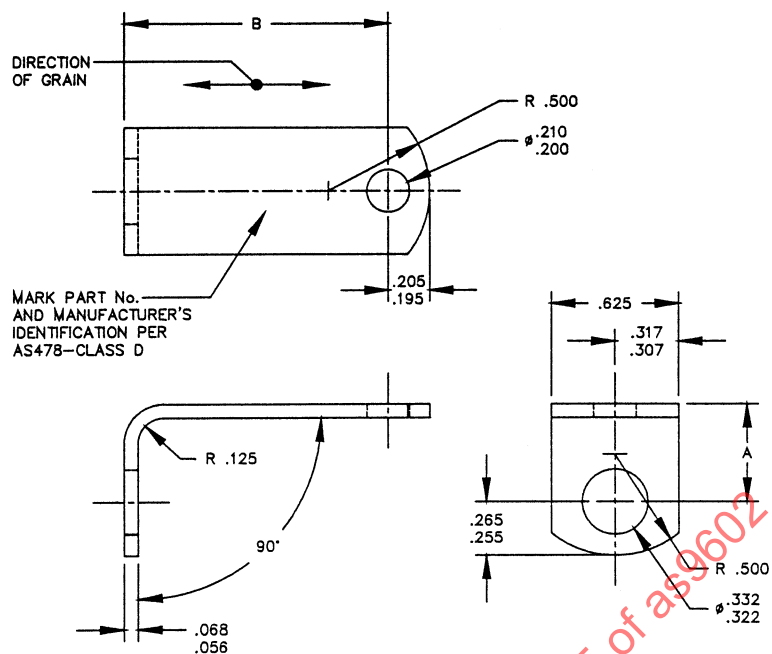
FIGURE 1 - ANGLE BRACKET
