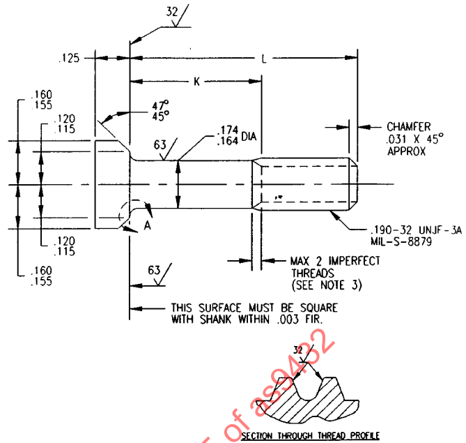
FIGURE 1 - BOLT
