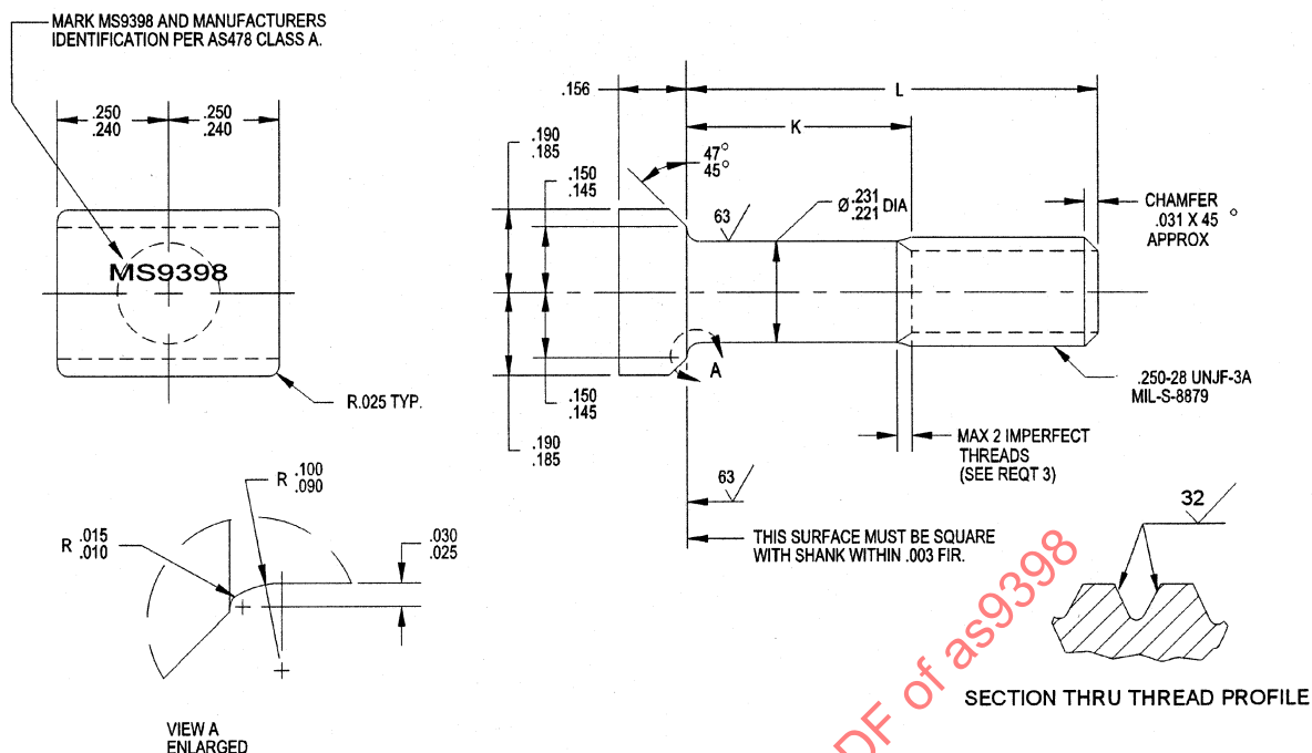
FIGURE 1 - BOLT
