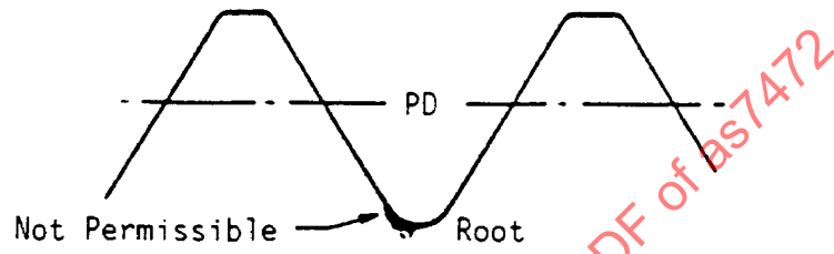
FIGURE 4 - Root Defects, Rolled Thread
