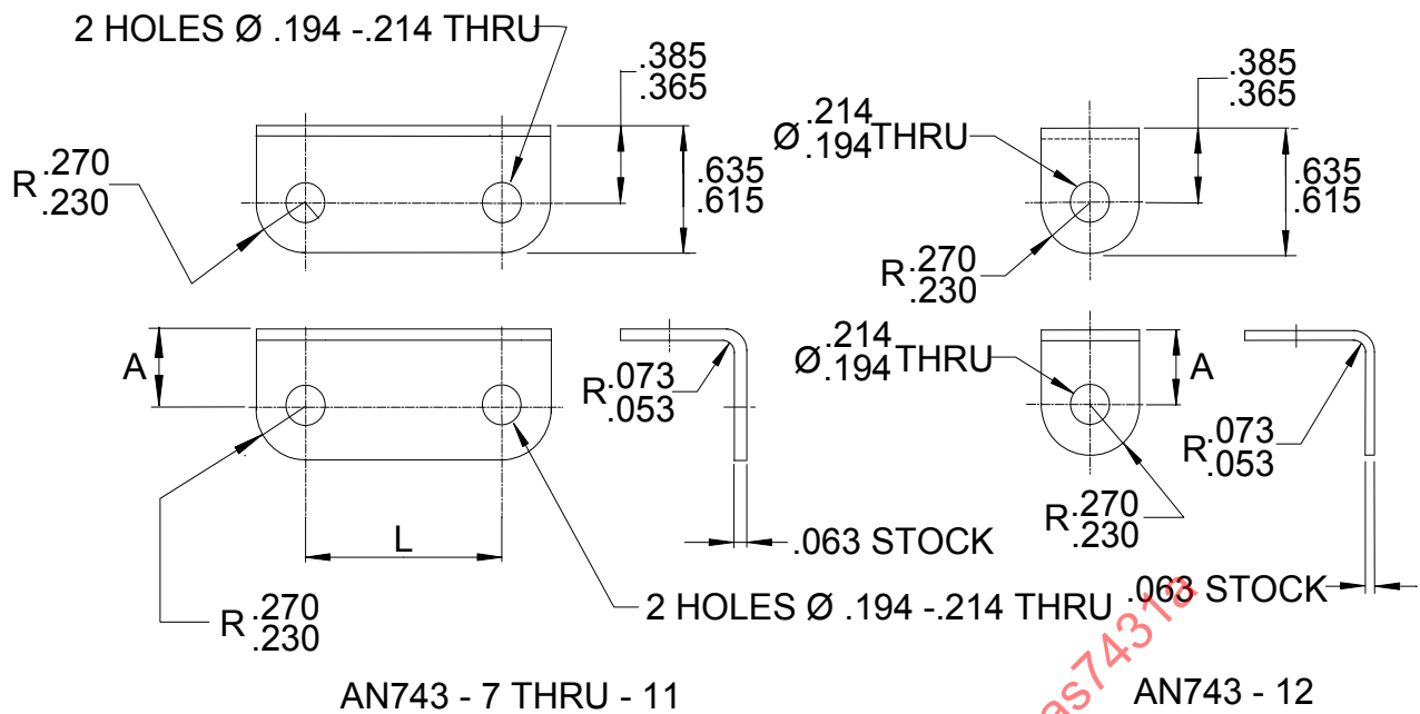
FIGURE 1 - BRACKETS (CONTINUED)
