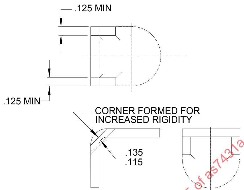
FIGURE 1 - BRACKETS (CONTINUED)
