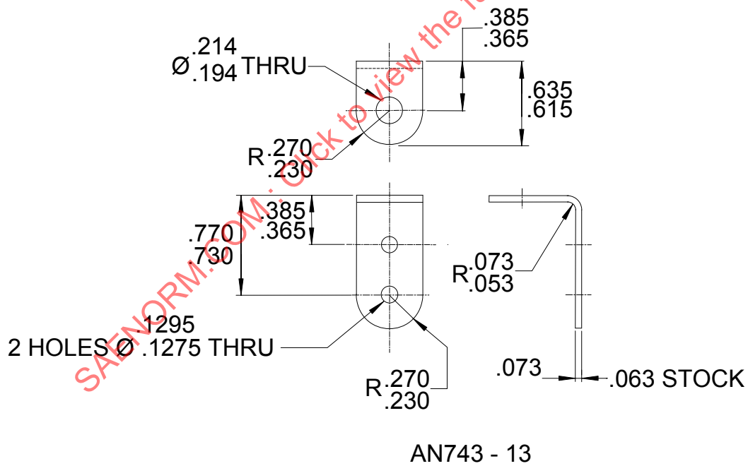
FIGURE 1 - BRACKETS (CONTINUED)
