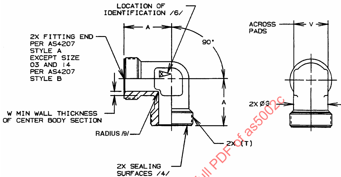
FIGURE 1 - FITTING, ELBOW, 90°
