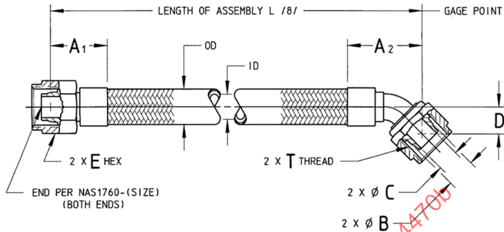
FIGURE 1 - HOSE ASSEMBLY
