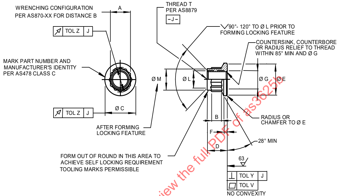
FIGURE 1 - NUT
