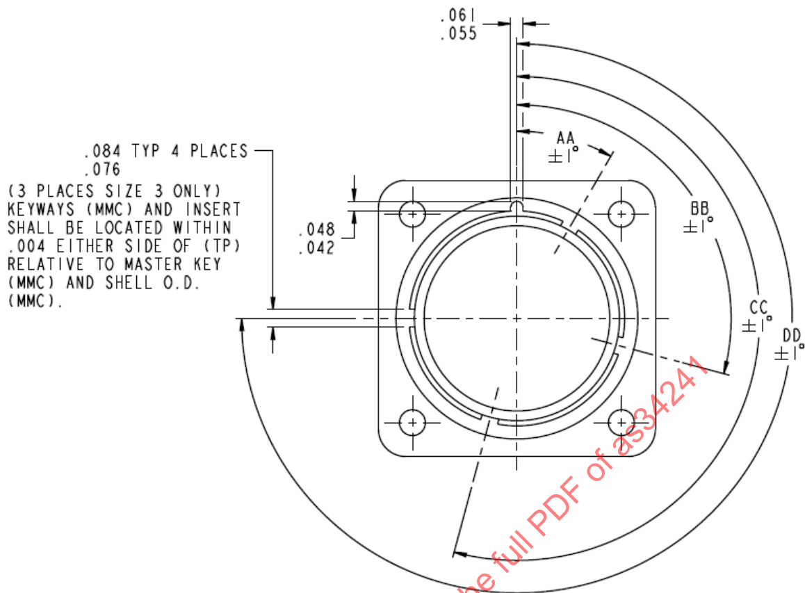
FIGURE 3 - KEYWAY POSITION
