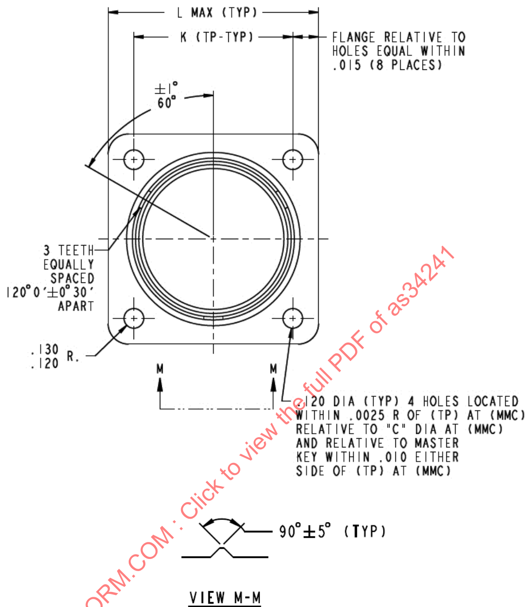
FIGURE 1A - CONNECTOR CONFIGURATION AND DIMENSIONS
