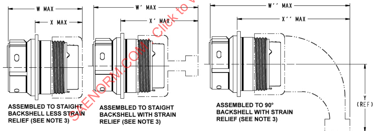
FIGURE 4 - BACKSHELL ACCESSORIES
