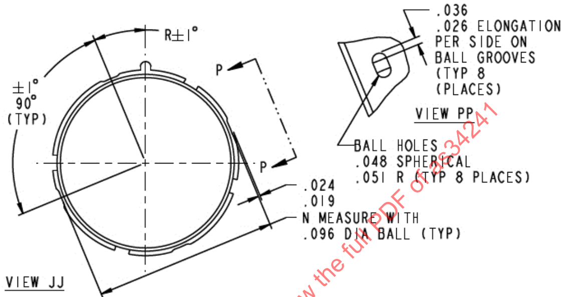
FIGURE 1D - CONNECTOR CONFIGURATION AND DIMENSIONS
