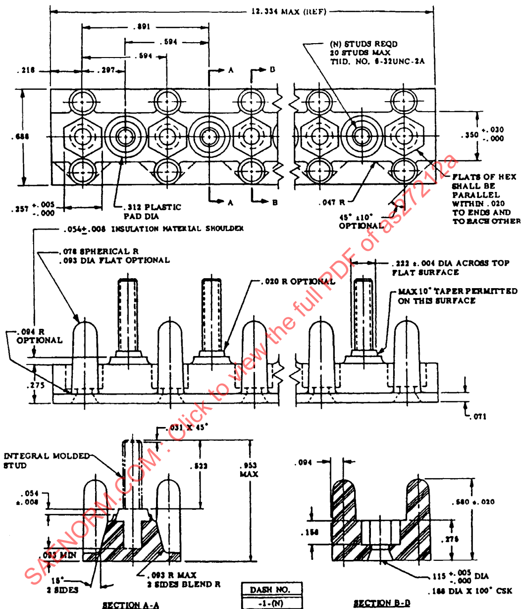
FIGURE 1 – MS27212-1-N TERMINAL BOARD
