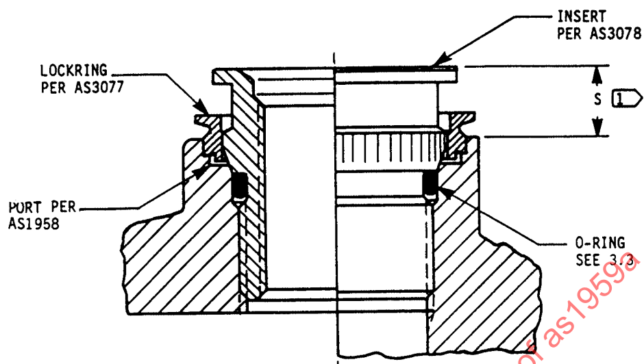
FIGURE 1 - Installed Insert and Lockring
