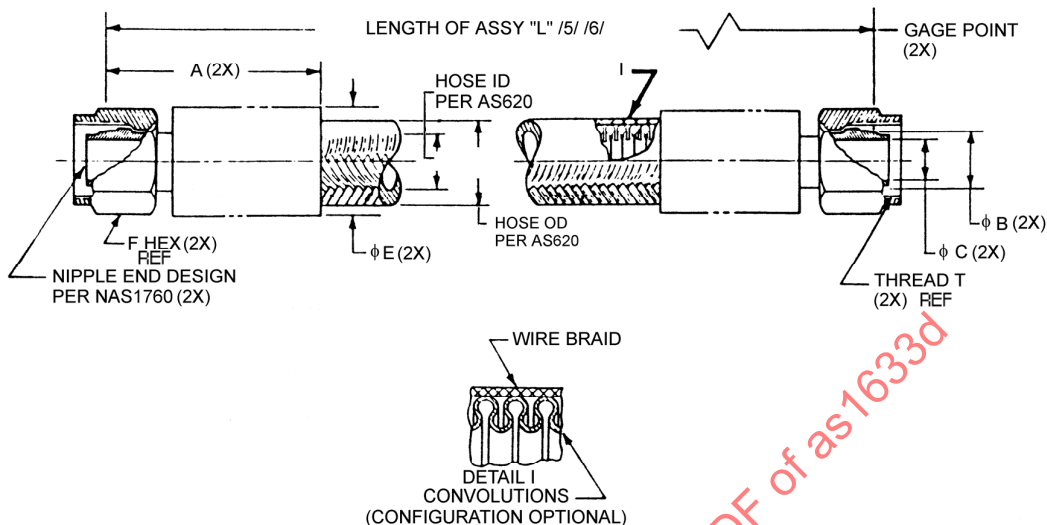
FIGURE 1 - HOSE ASSEMBLY
