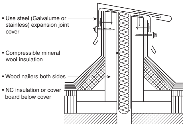
FIGURE 38.12.1.3 Expansion Joint.
