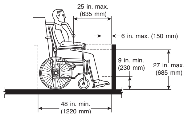
FIGURE 12.45.8.2.4.7 Protrusions in Wheelchair Spaces in Amusement Rides. [ADA/ABA-AG: Figure 1002.4.4.3]
