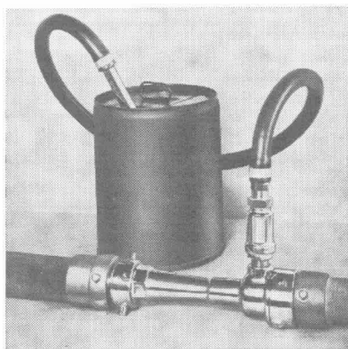
Fig. A-121 (b) (1) (a). In-Line Inductor.
