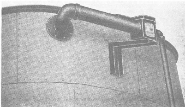
Fig. A-3411 (a). Air Foam Maker in Horizontal Position at Top of Storage Tank.
