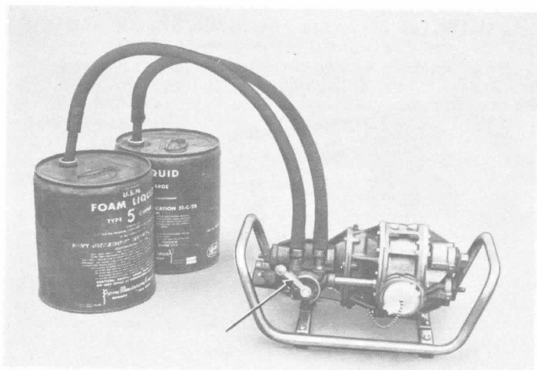
Fig. A-121(f). Coupled water motor pump proportioner.
