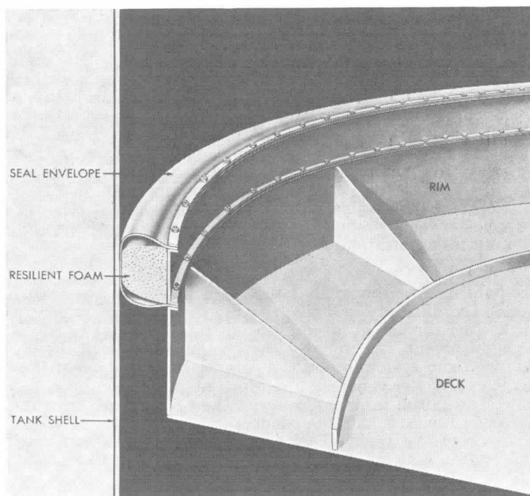
Fig. A-3413. Seal on floating metal pan of covered floating roof tank.
