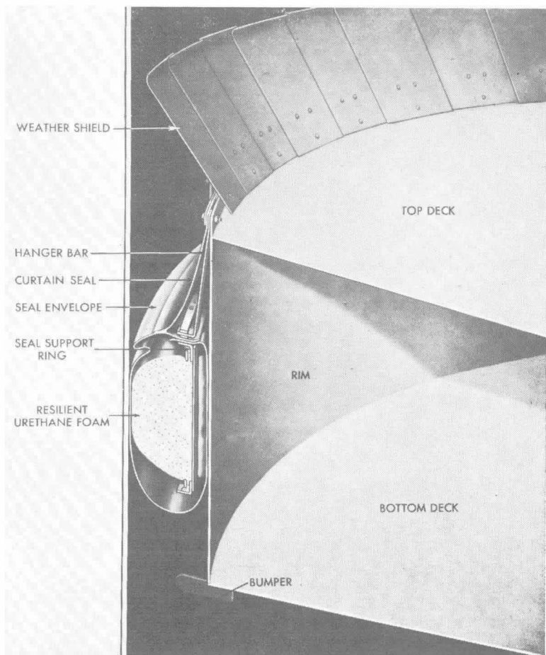
Fig. A-3412(2). Tube seal-open floating roof tank.
