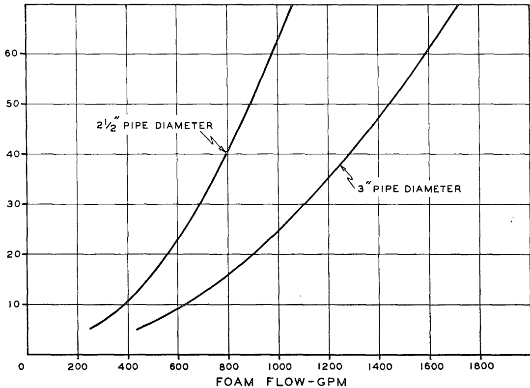
FRICITION LOSSES — PSI PER 100 FT. OF PIPE Fig. A-352A
