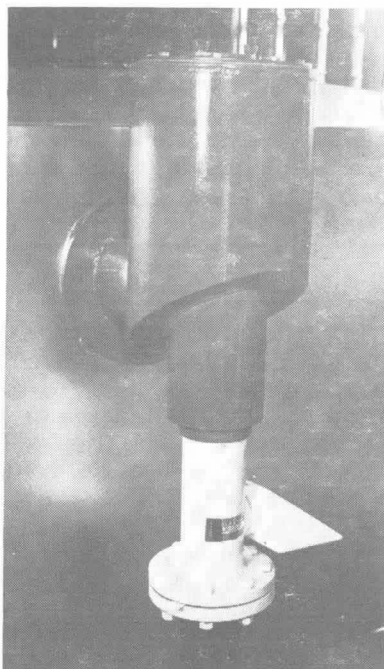
Fig. A-3411 (b). Foam chamber and foam maker.
