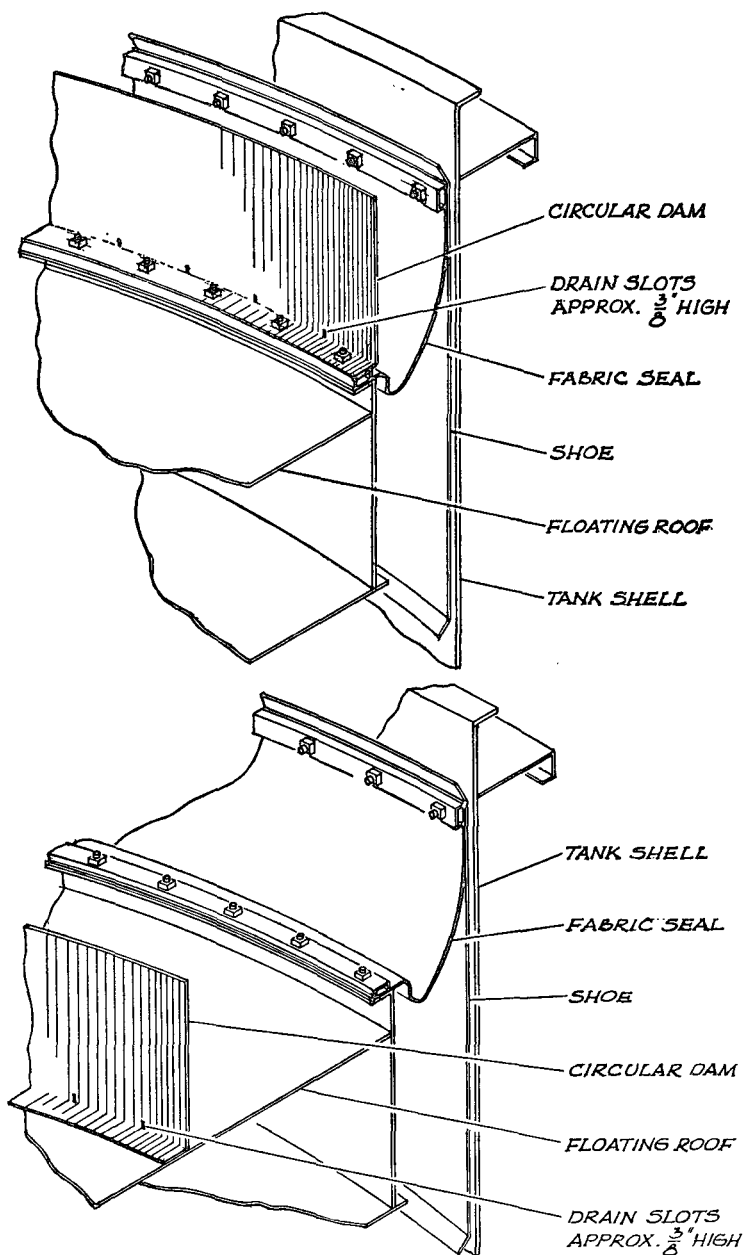
Fig. A-3412(3). Typical Foam Dams for Floating Roof Tank Fixed Protection.
