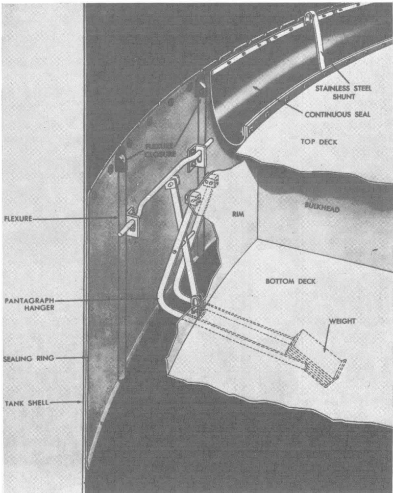
Fig. A-3412(1). Pantograph type seal-open top floating roof tank.
