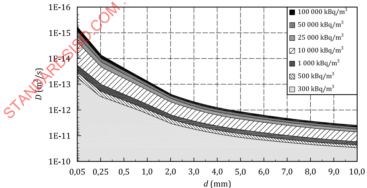
Figure 8 — Minimum radon activity concentration in the source container
