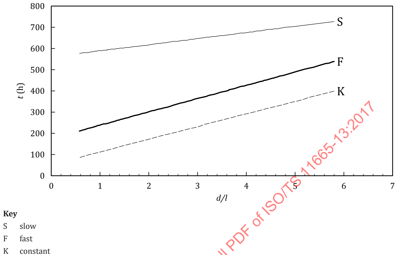
Figure 7 — Minimum duration of the decisive measurement for non-stationary radon diffusion
