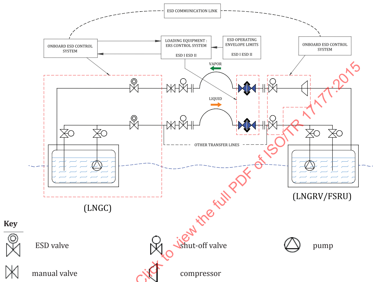
Figure A.2 — Side to side or side by side (refer to Figure B.2 and Figure B.6 )
