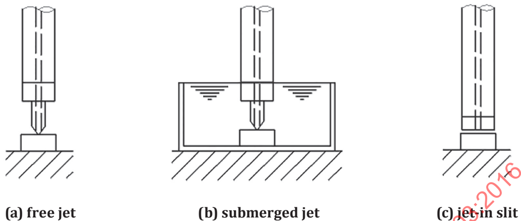
Figure 5 — Impinging jets used to evaluate localized corrosion
