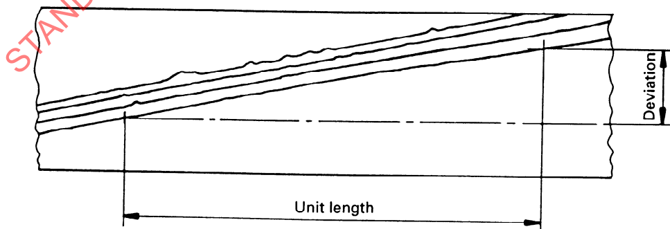
Figure 4 — Measurement of slope of grain
