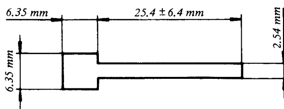
FIG. 2 – Modified T-50 test piece Test piece thickness : 2.0 \pm 0.2 mm
