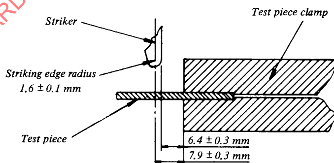
FIG. 1 — Test piece clamp and striker
