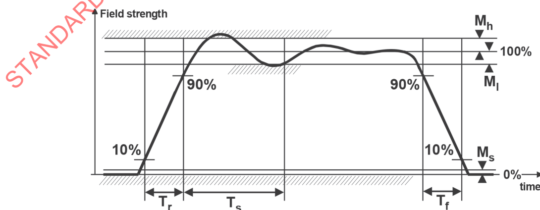
Figure 6.3 — Interrogator power-up and power-down RF envelope
