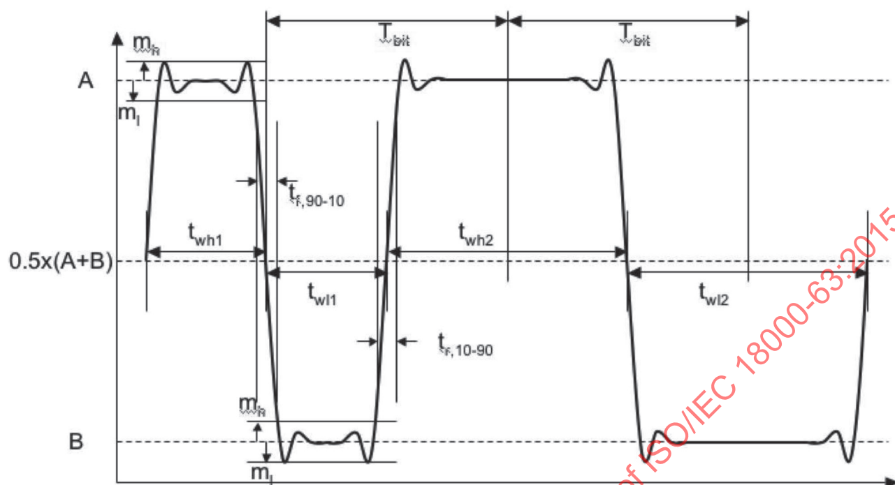
Figure 7.29 — Manchester waveform
