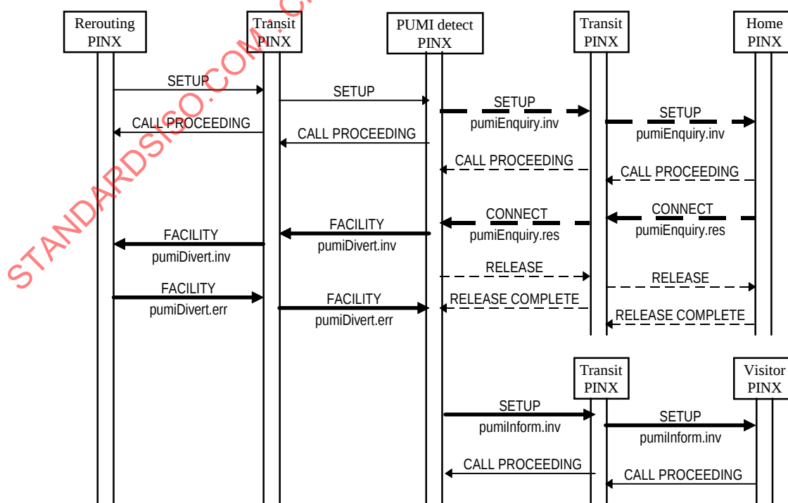
Figure C.2 - Example of forward switching by the PUMI-detect PINX
