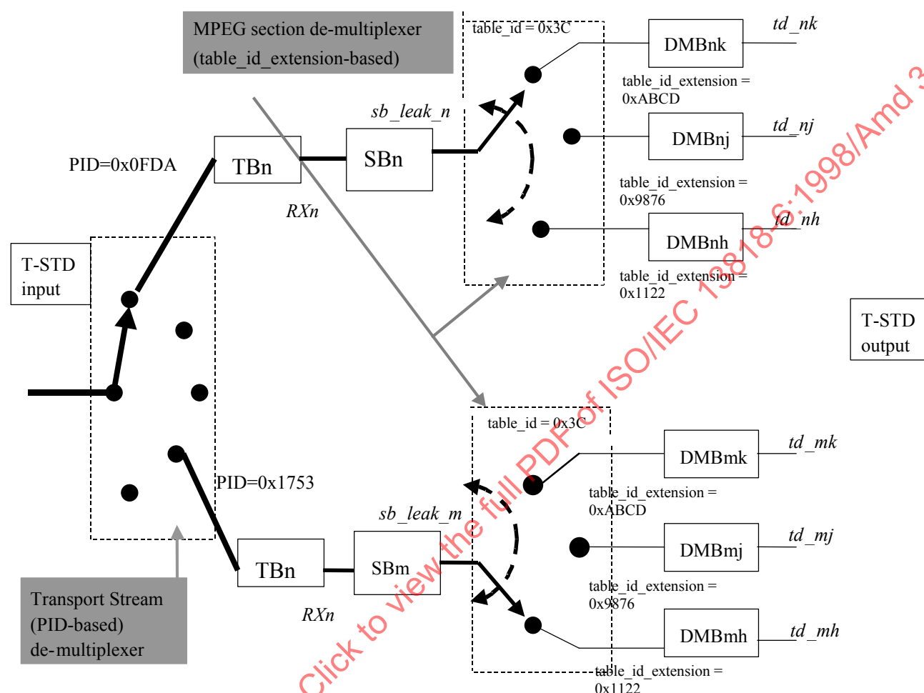
Figure 9-1 T-STD for DSM-CC Synchronized Download Protocol
