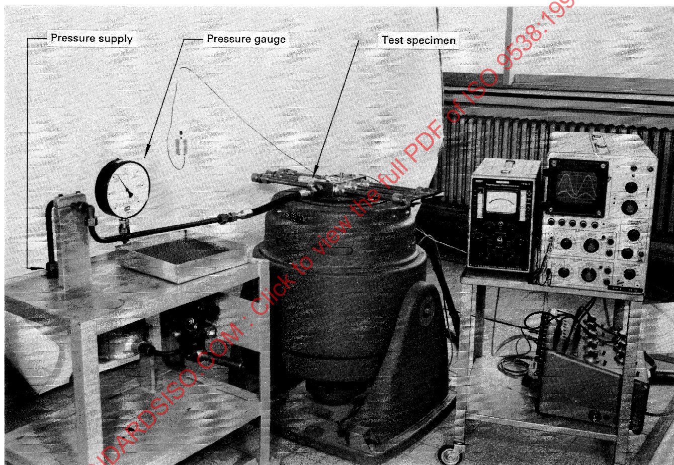
Figure 1 — Set-up of test drive
