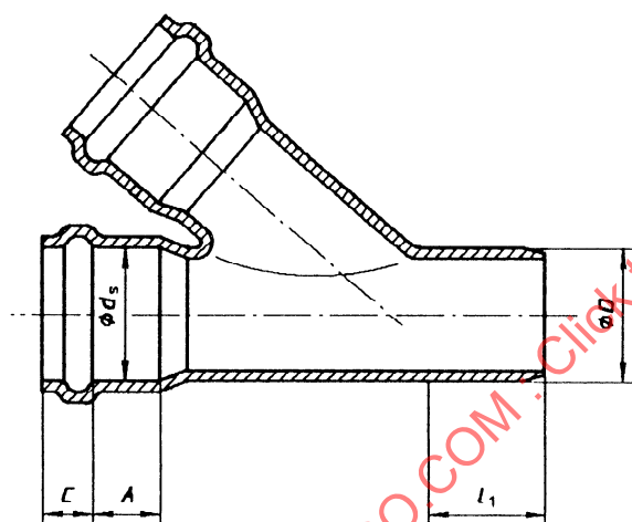
Figure 3 — Basic dimensions
