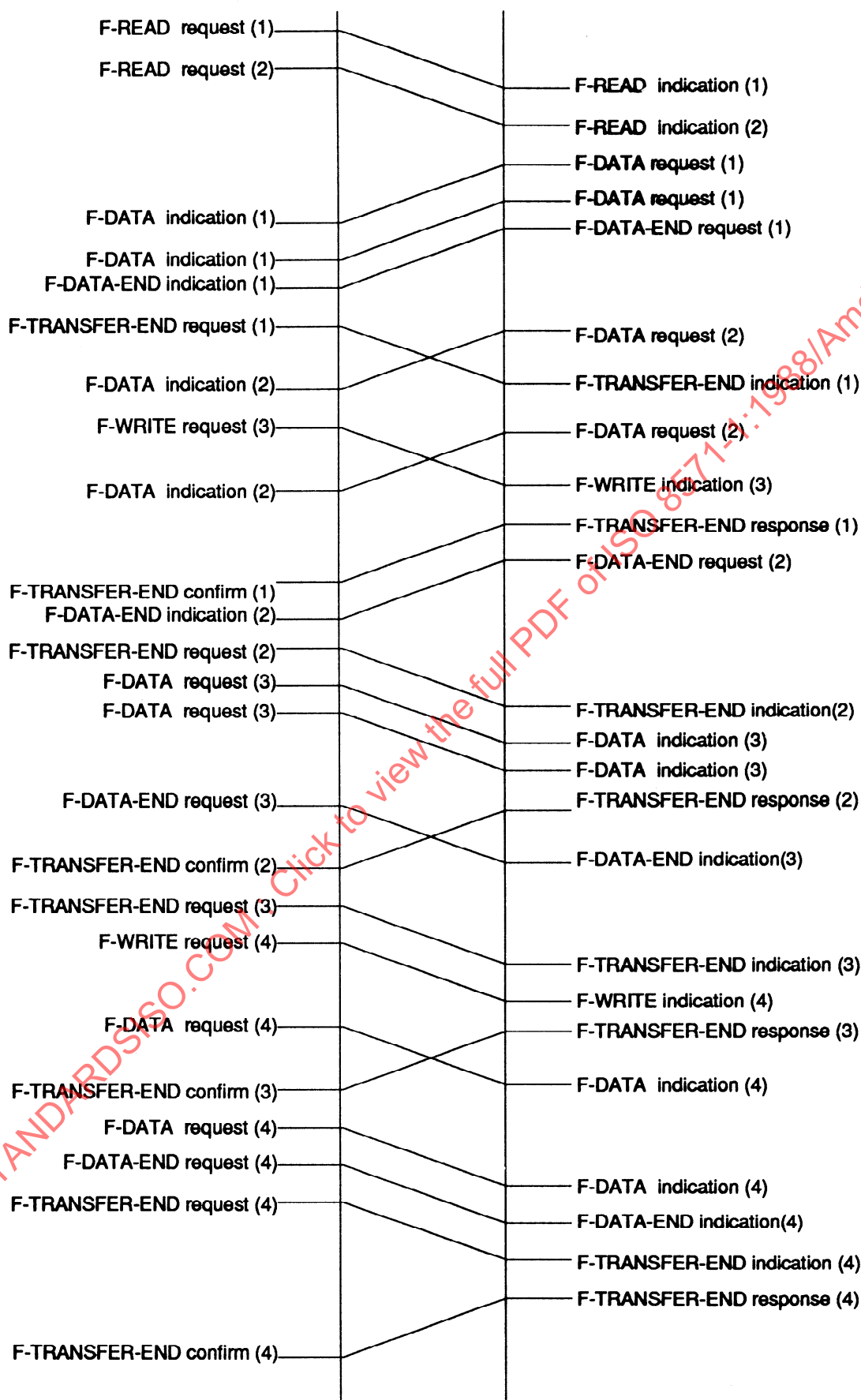
Figure 15 - Use of FTAM in a LAN fileserver with consecutive access
