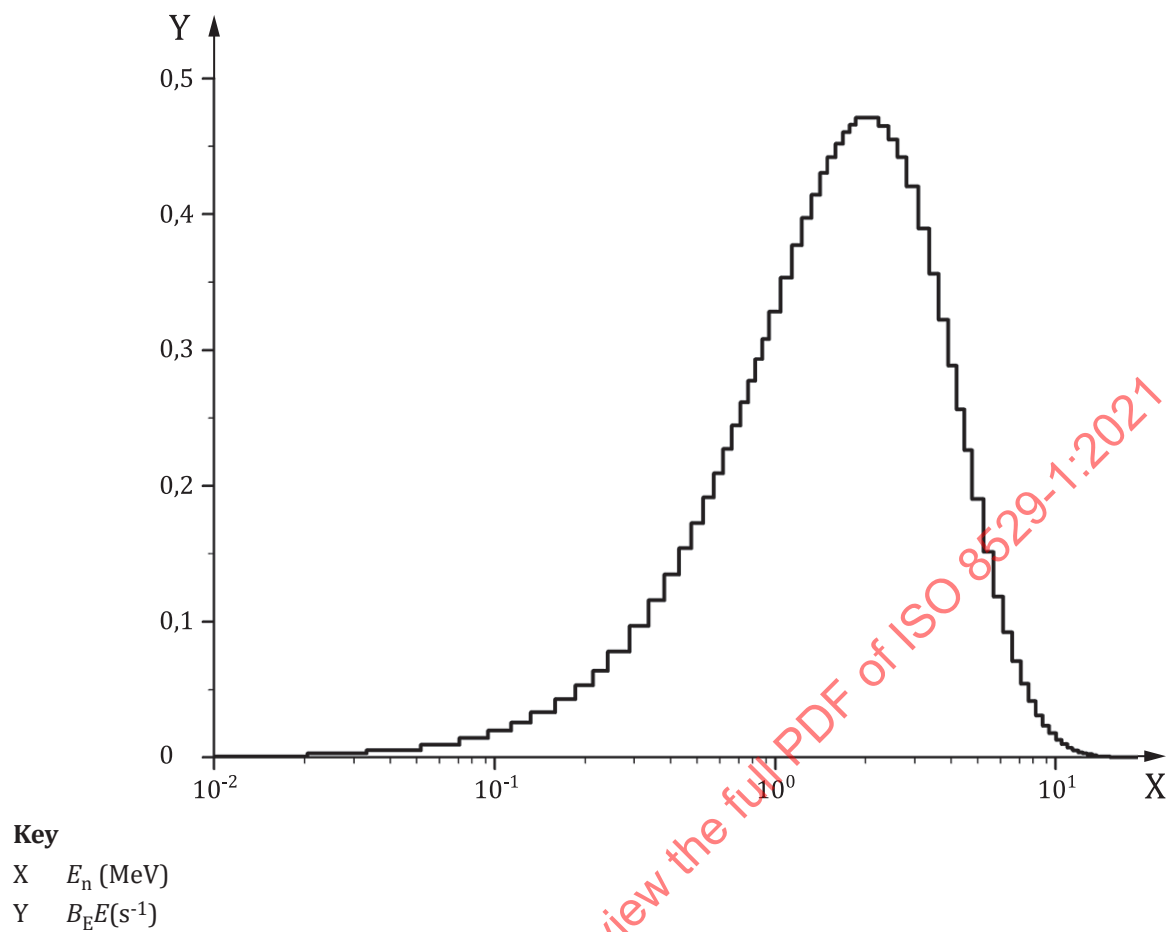
Figure B.1 — Neutron spectrum from a ^{252}\text{Cf} spontaneous fission source
