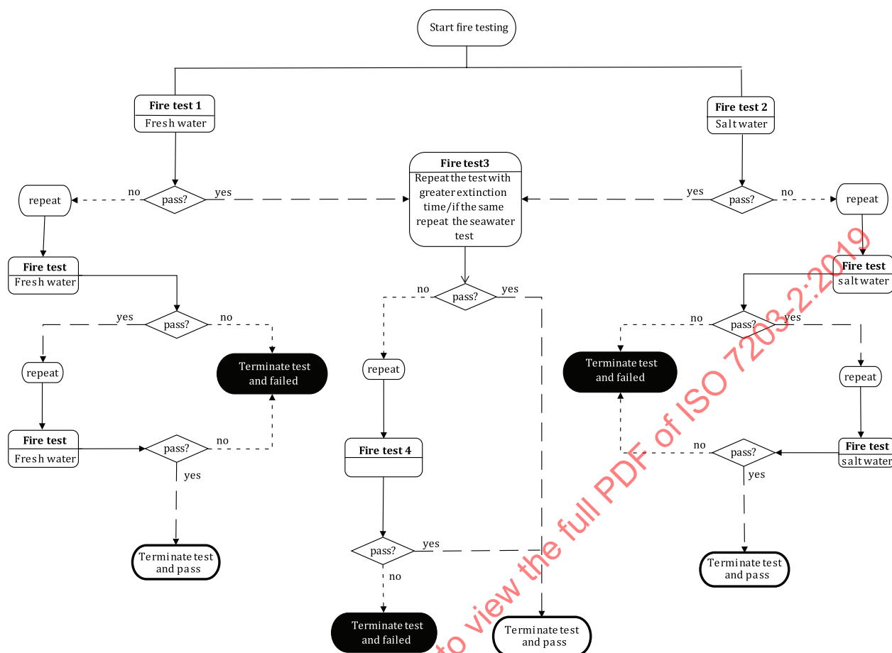
Figure I.1 — Decision tree for fire performance test on water-immiscible fuels
