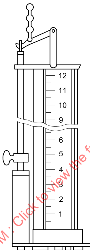
Figure 7 — Thief sampler
