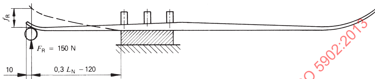
Figure 6 — Determination of rear spring constant, c_R
