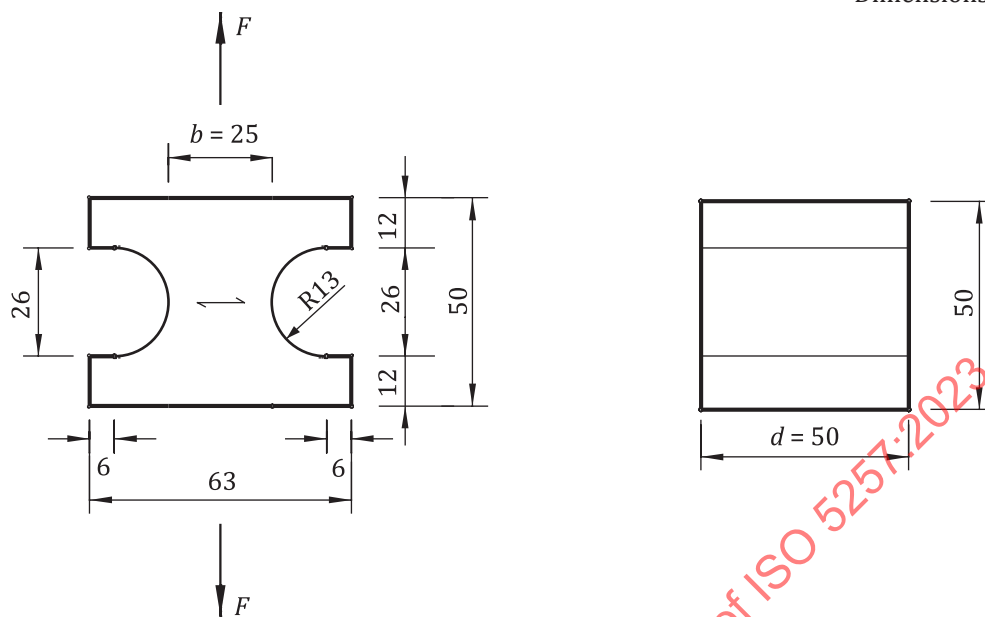
Figure 6 — Perpendicular-to-fibre tensile test specimen schematic
