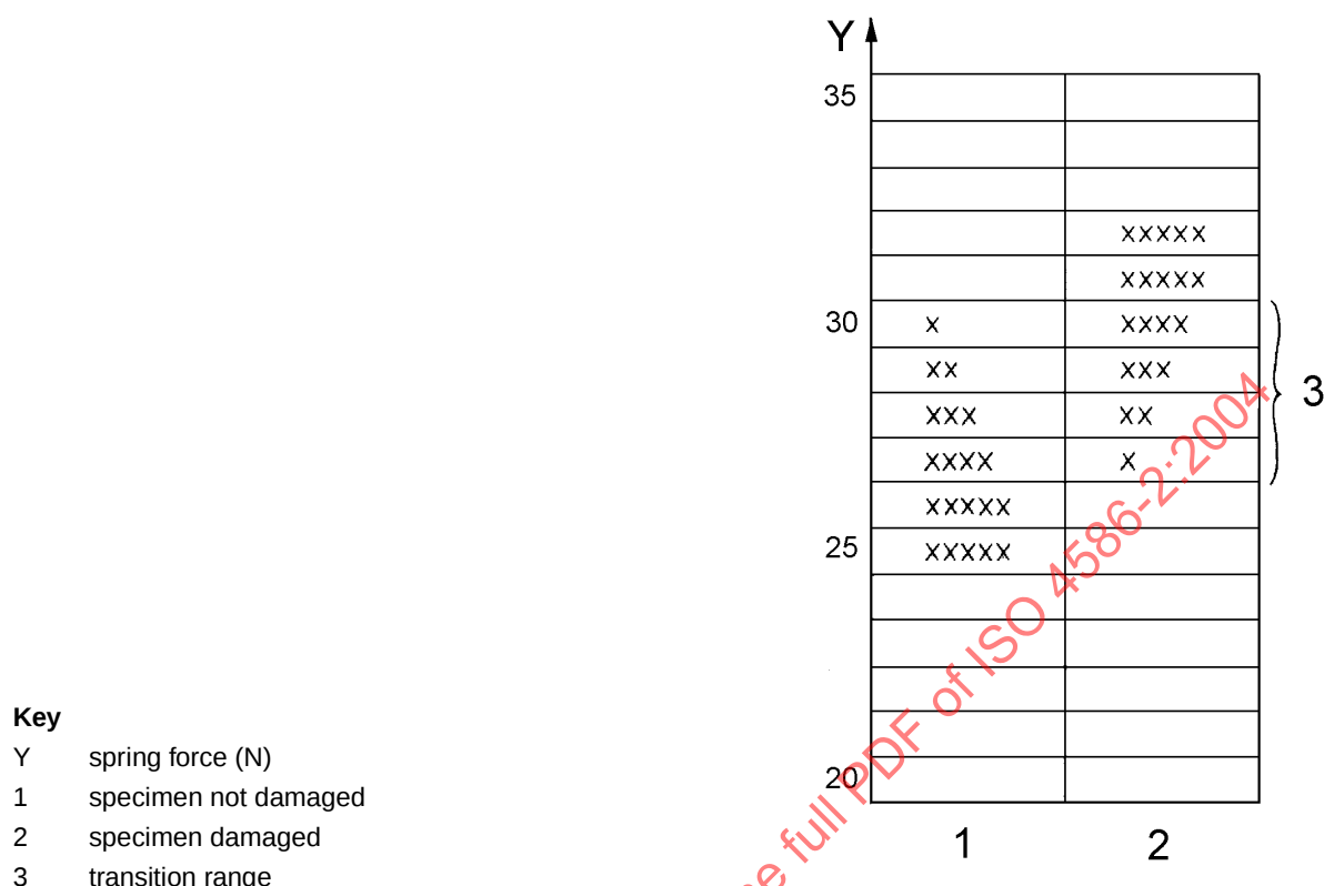
Figure 7 — Example of evaluation diagram for assessing the effect of impact blows with an impact tester (see 12.7)
