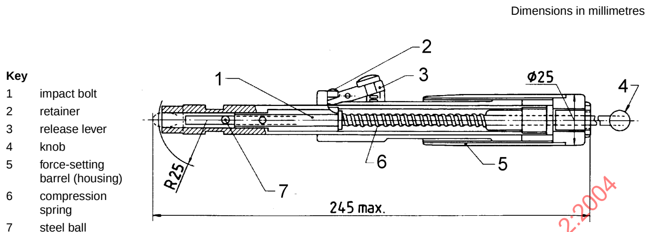
Figure 4 — Impact tester (shown with spring compressed) (see 12.3.1)
