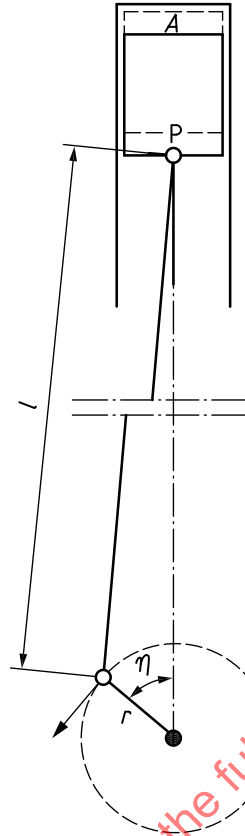
a) Conventional crankshaft with connecting rod and small end
