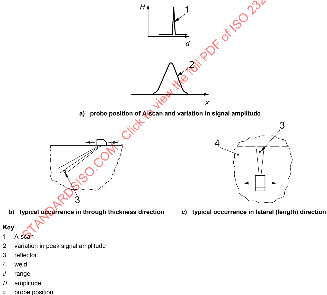
Figure C.1 — Pattern 1 ultrasonic response
