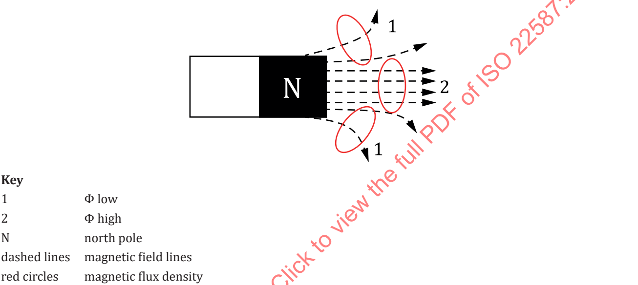
Figure A.1 — Magnetic flux density distribution
