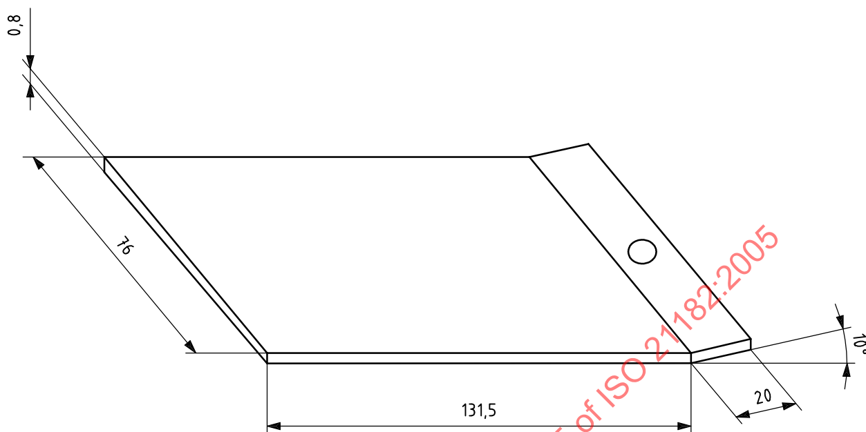
Figure 2 — Metallic test panel
