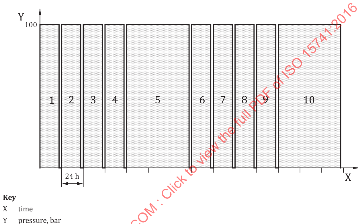
Figure C.1 — Complete set of pressure cycles
