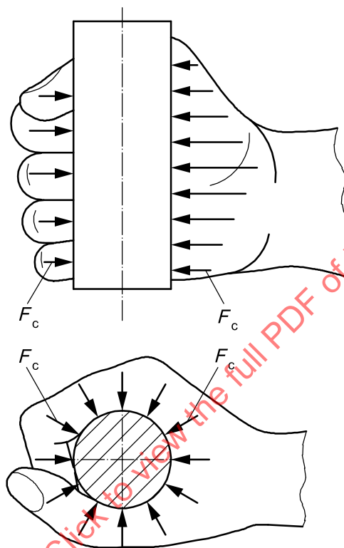
Figure 7 — Example of contact forces, F_c
