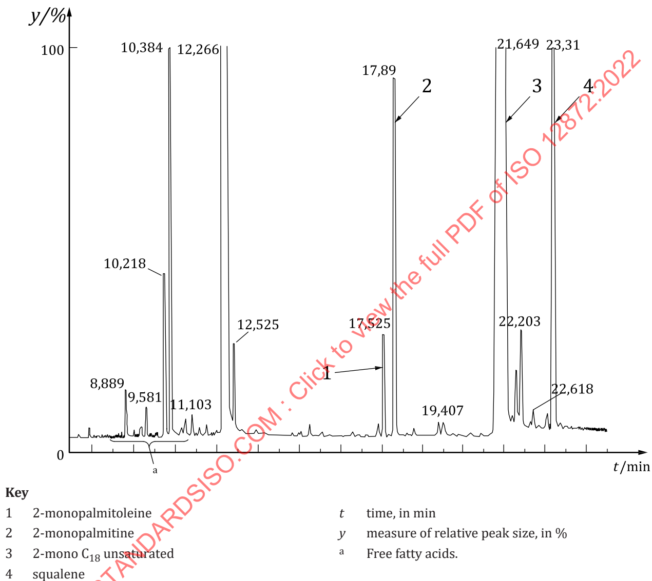
Figure A.1 — Chromatogram of the silylation reaction products obtained by lipase action on a refined olive oil spiked with 20 % volume fraction esterified oil
