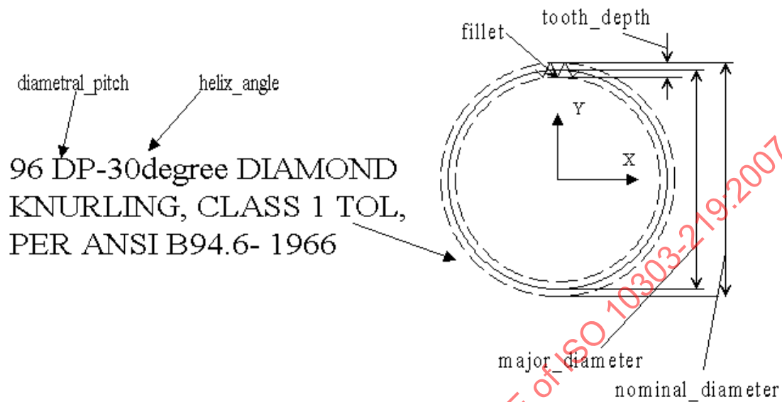
Figure 141 — Turned knurl
