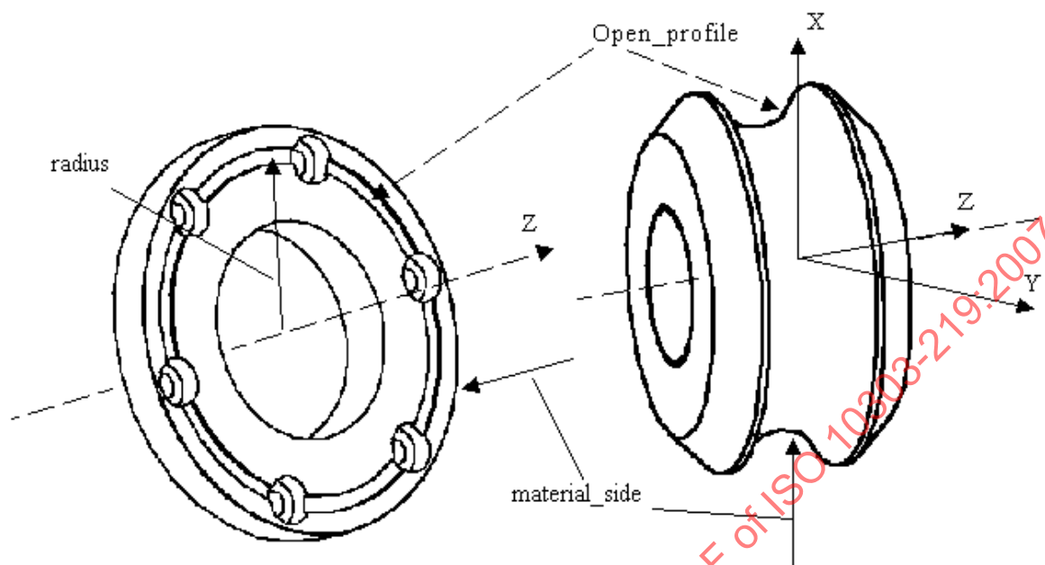
Figure 85 — Groove
