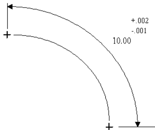
Figure 43 — Distance_along_curve_tolerance
