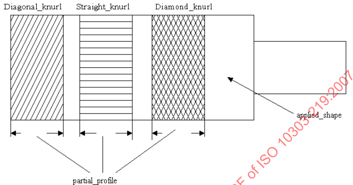
Figure 90 — Knurl and types of Turned_knurl
