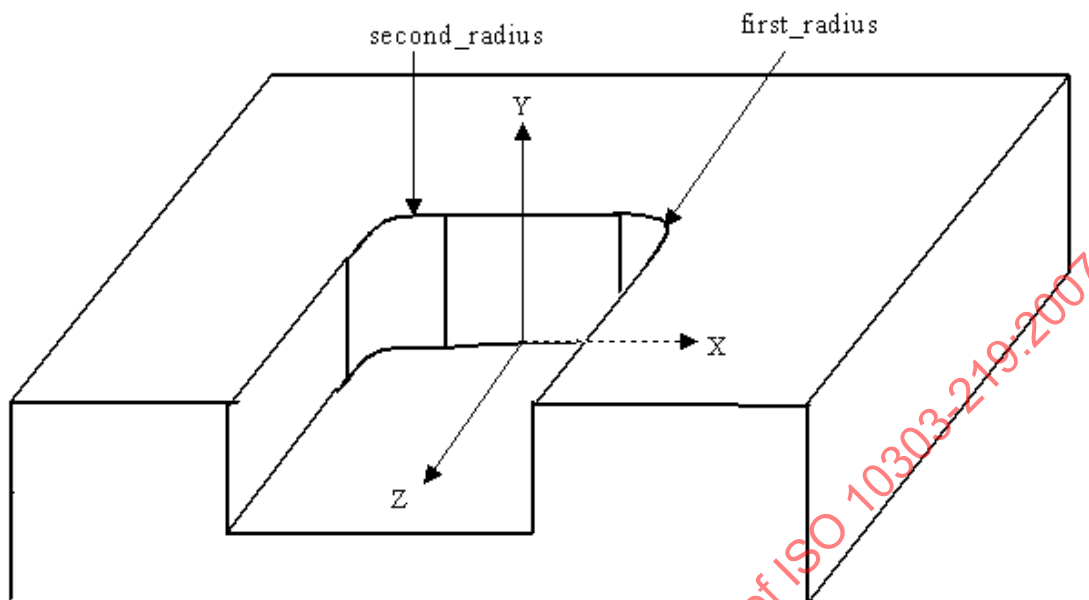
Figure 67 — Flat_slot_end_type
