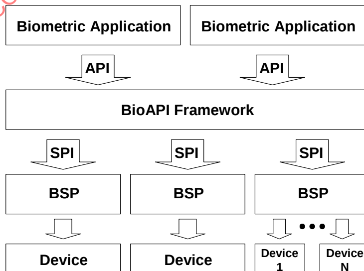
Figure 2: BioAPI architecture
