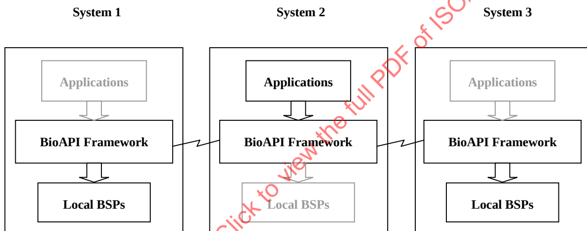
Figure 3: Use of the BIP for communication between systems
