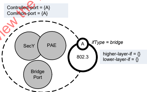
Figure 14-9—Augmented Interface Model of Bridge Port with a PAE
