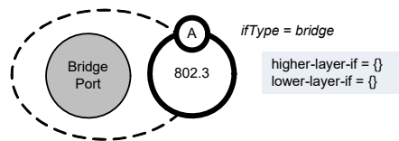
Figure 14-6—Augmented Interface Mode of Bridge Port
