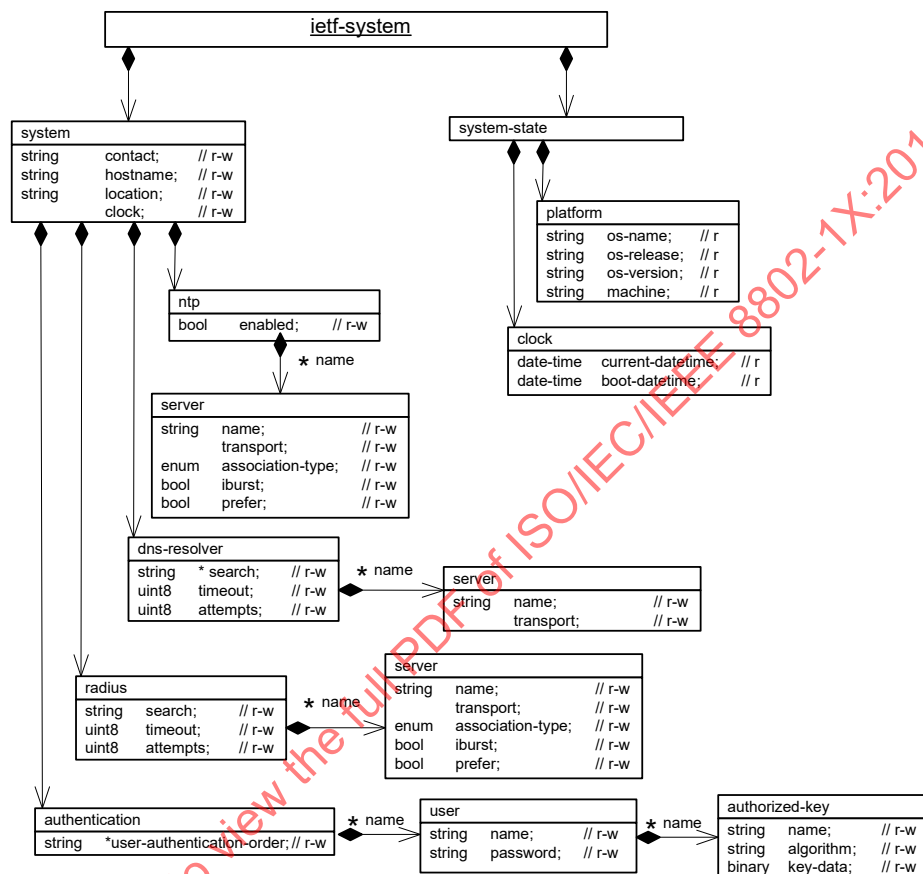
Figure 14-3—IETF System Management YANG data model
