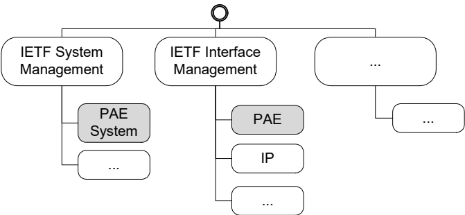
Figure 14-2—YANG object hierarchy with IEEE Std 802.1X
