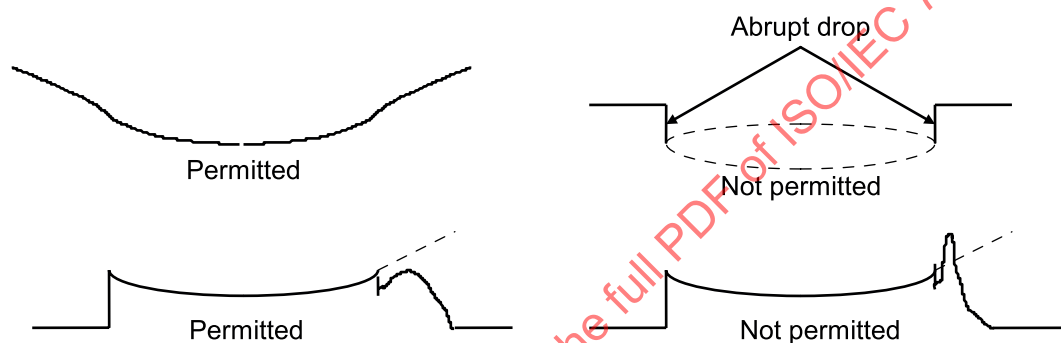
Figure 3 — Surface profile
