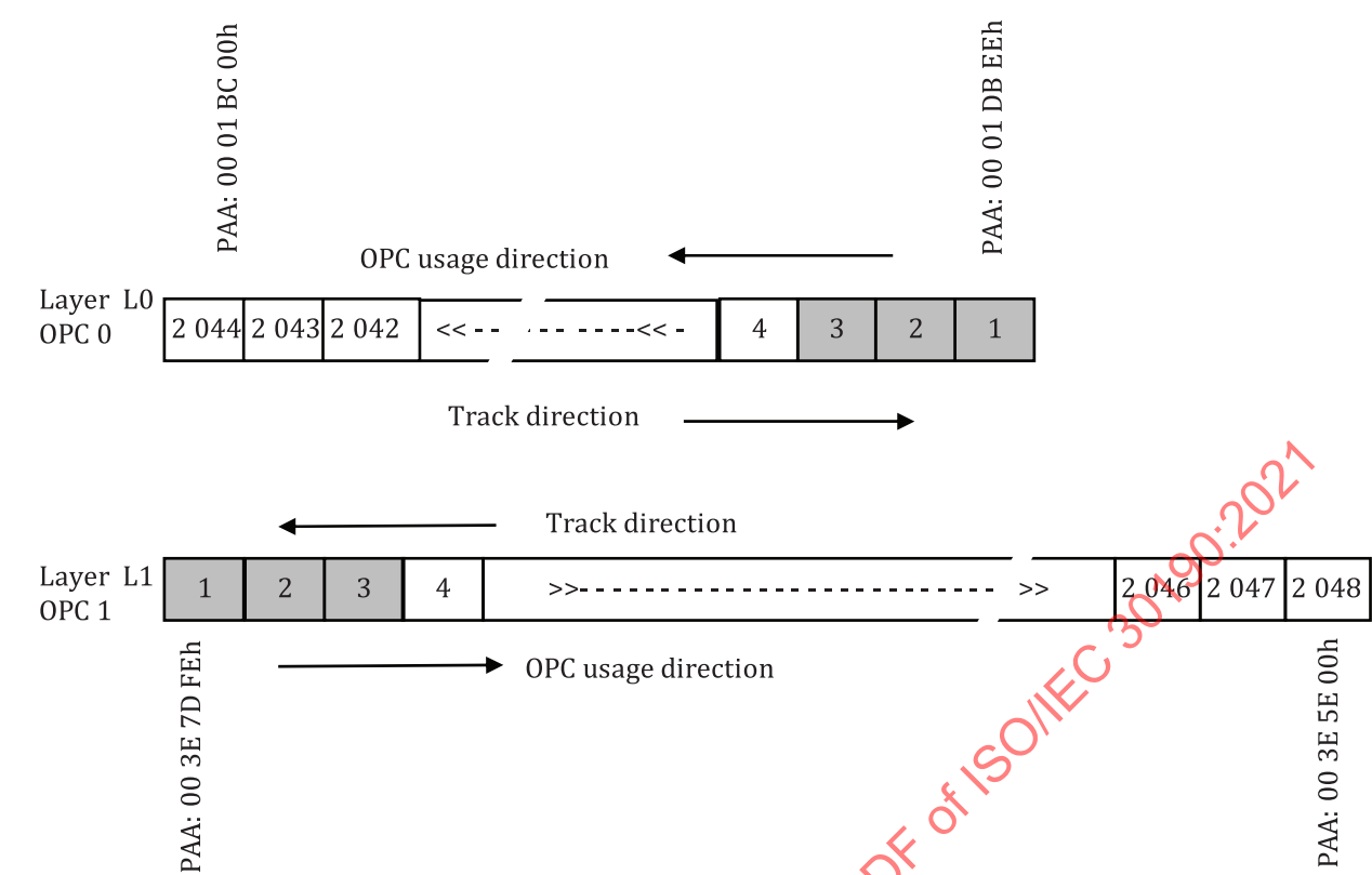
Figure 92 — Direction of usage of OPC area of layer L0 and layer L1
