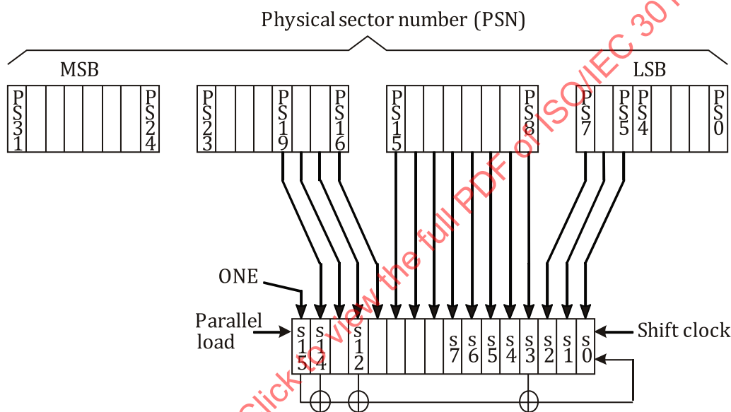
Figure 24 — Scrambler circuit
