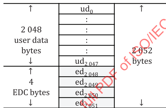
Figure 23 — Data frame
