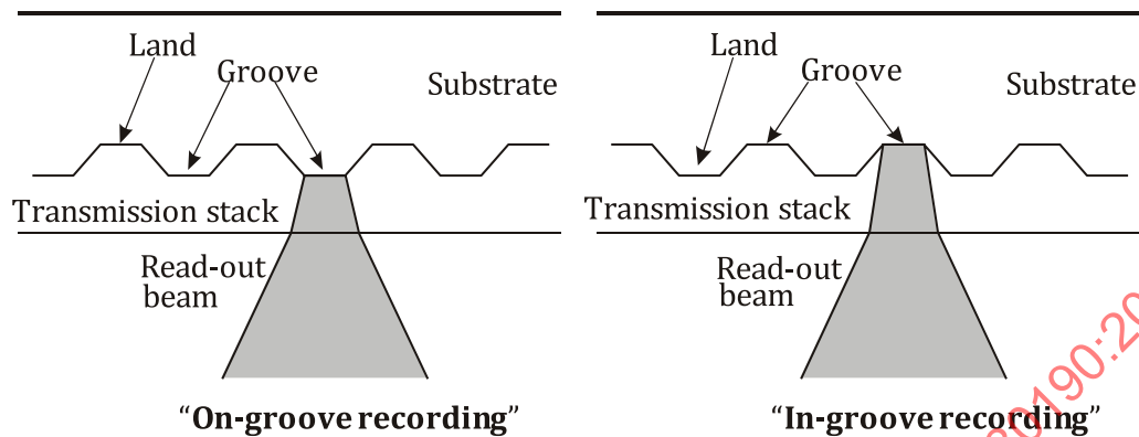
Figure 55 — Outline of groove geometry (radial cross-section of disk)
