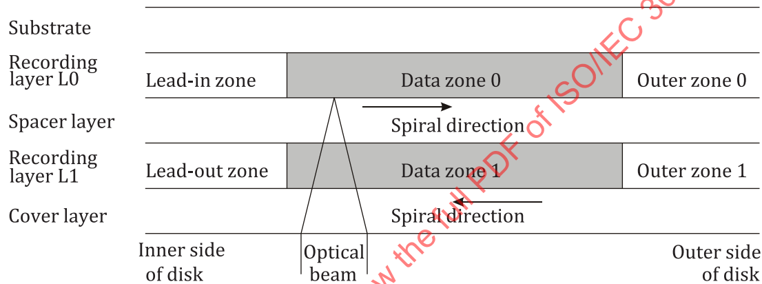
Figure 18 — Subdivision of information zone on DL disk
