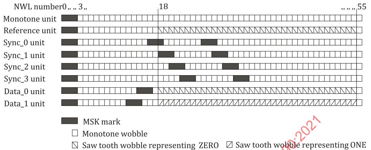
Figure 67 — ADIP unit types
