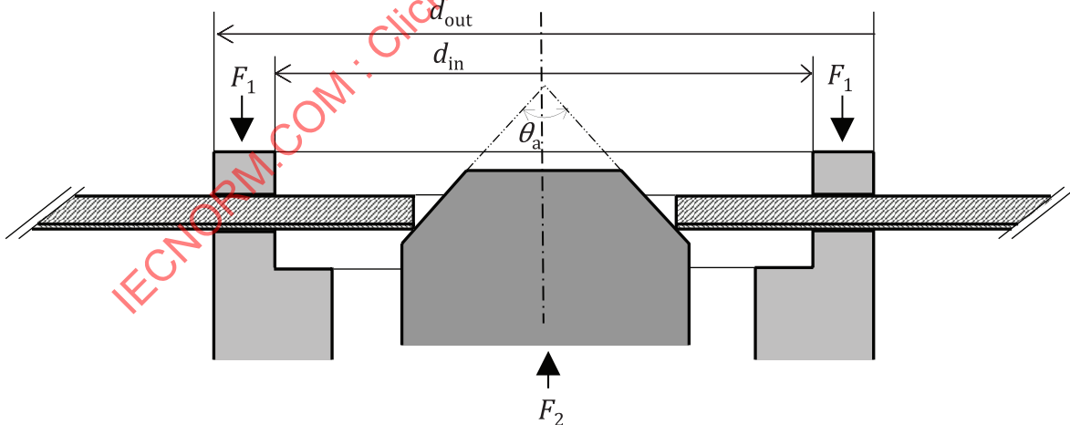
Figure 8 — Clamping conditions for measurement
