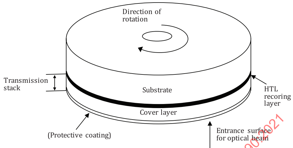
Figure 1 — Outline of type SL/HTL disk
