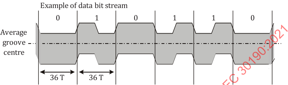
Figure 60 — Biphase modulated HFM groove
