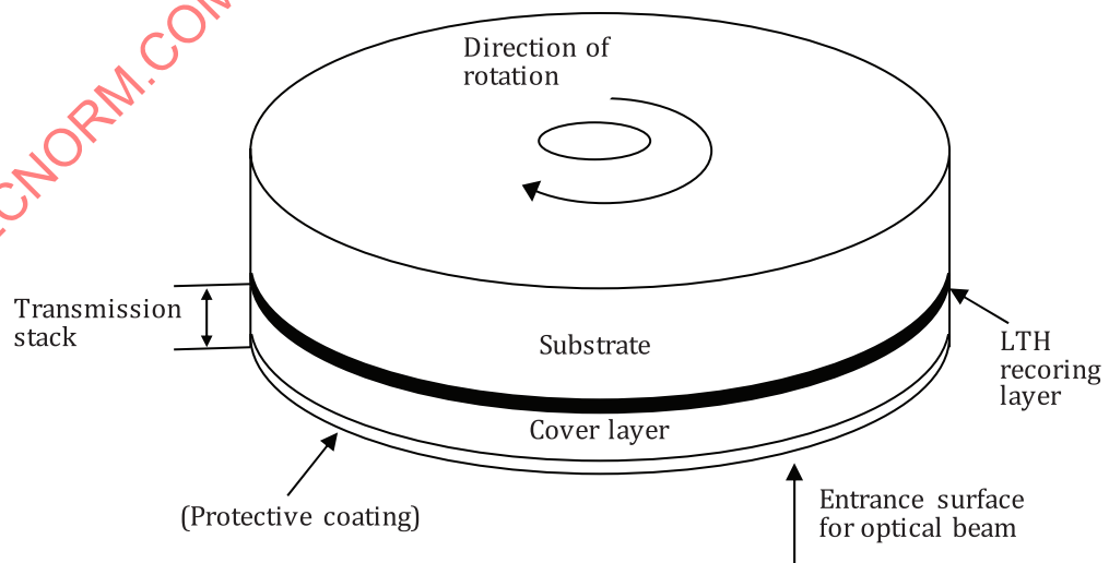
Figure 3 — Outline of type SL/LTH disk
