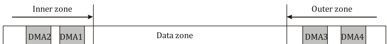
Figure 119 — Disk management areas
