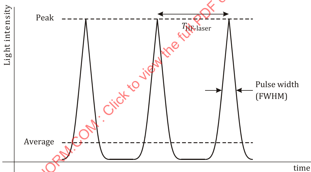
Figure 130 — Schematic representation of light pulses from Laser Diode
