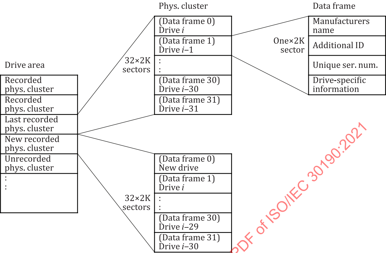
Figure 94 — Format of drive area (example)
