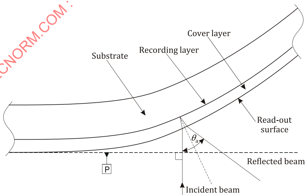
Figure 20 — Definition of angular deviation
