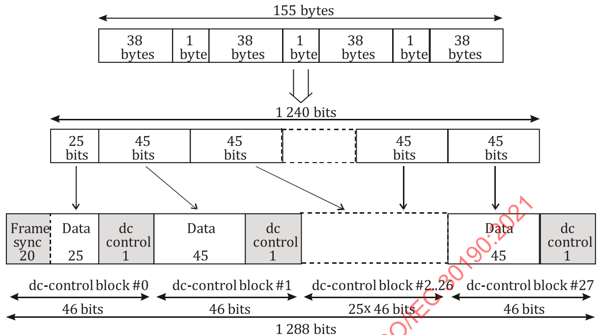
Figure 40 — Composition of recording frame
