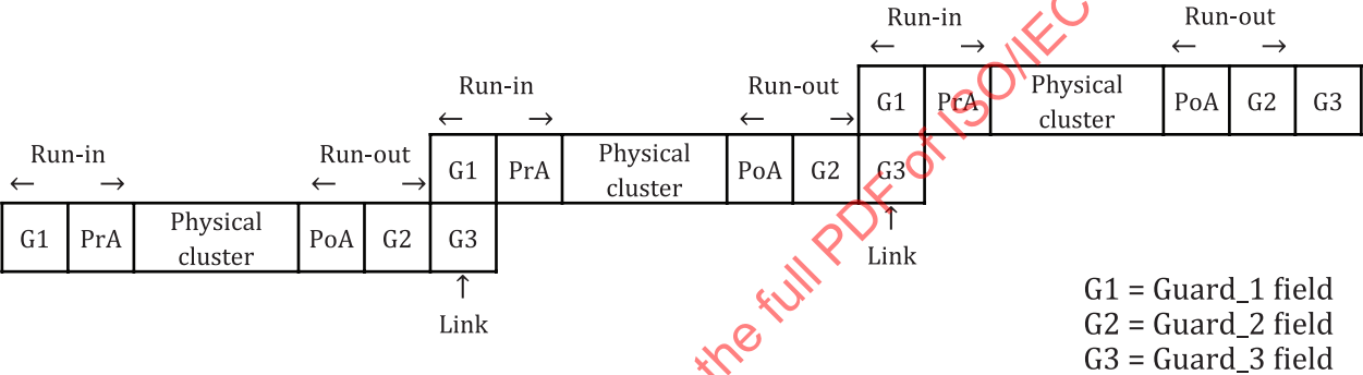
Figure 53 — Linking of 3 separately written single recording unit blocks
