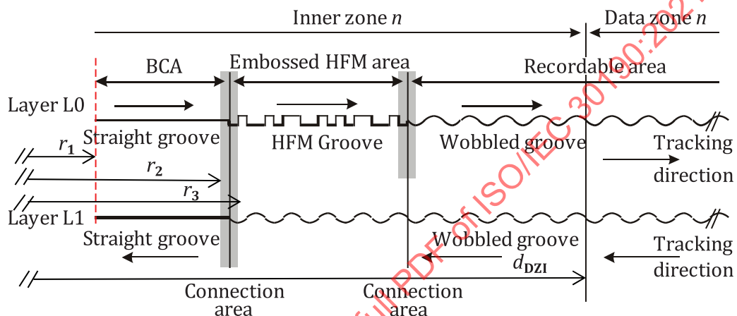
Figure 54 — Connection areas between different groove types
