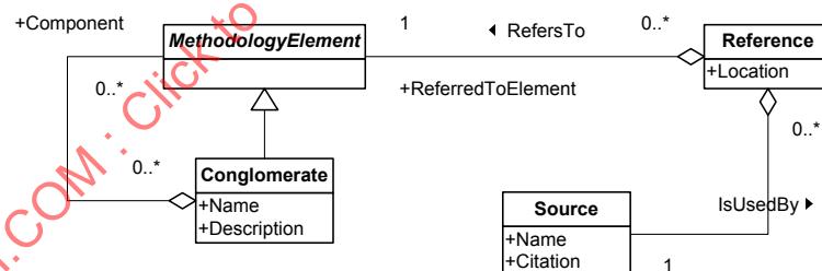
Figure 10 – Support classes
