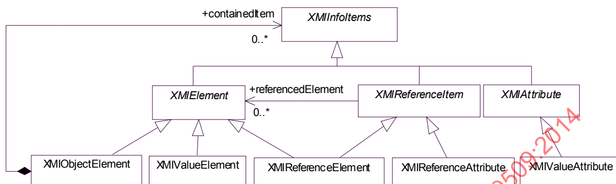
Figure 9.1- Serialization Model
