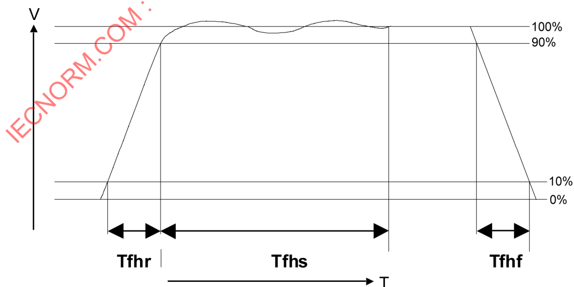
Figure 3 — FHSS carrier rise and fall characteristics
