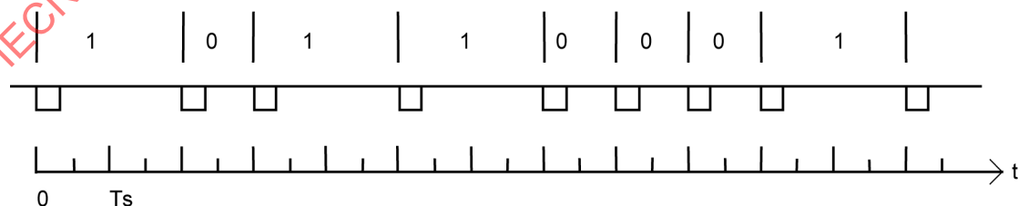
Figure 11 — Example of PIE byte encoding for 'B1'
