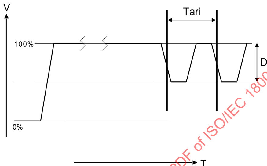
Figure 7 — Inter-pulse mechanism
